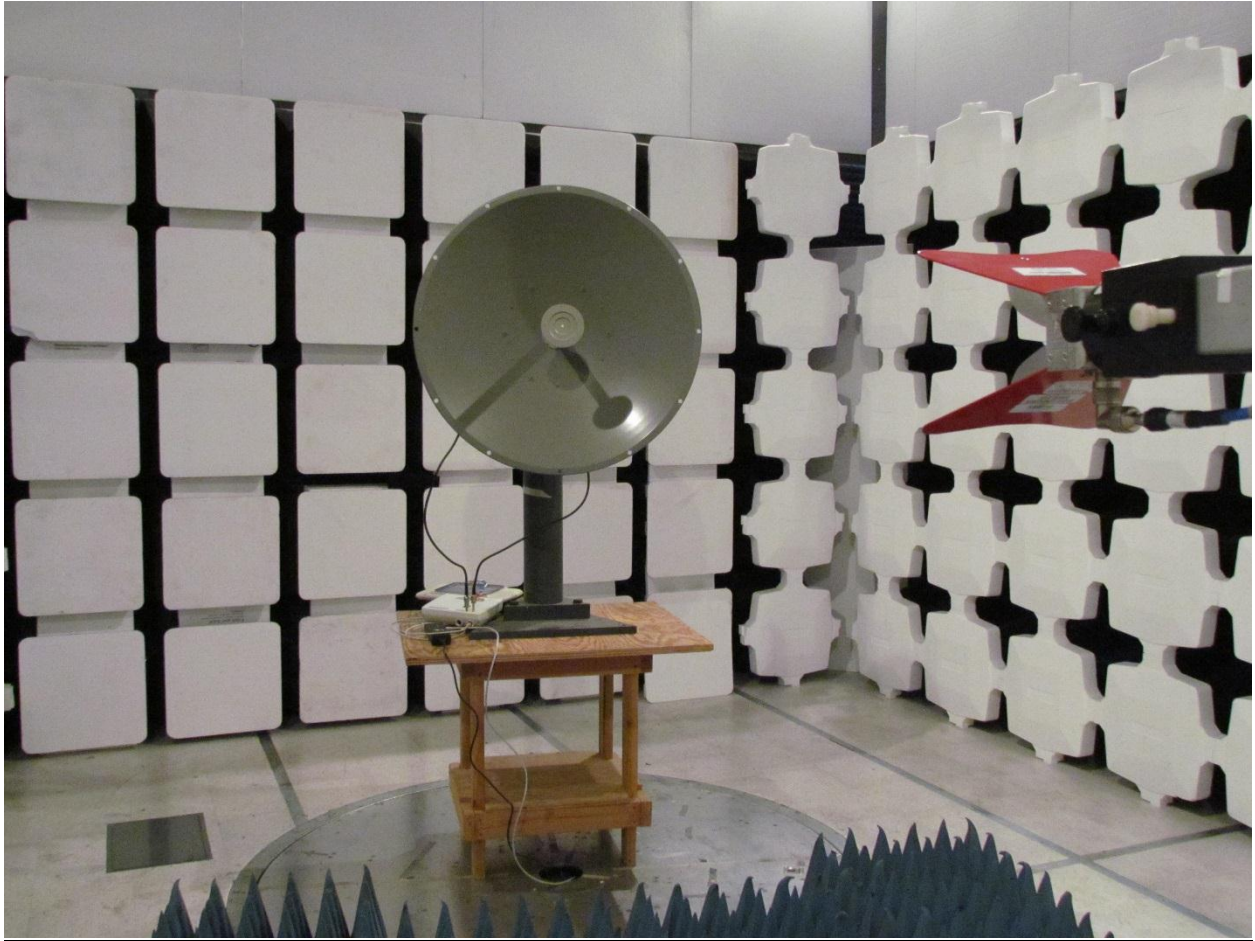
32 dBi Dish RW-9732-4958 TX Spur 1-18G Front
