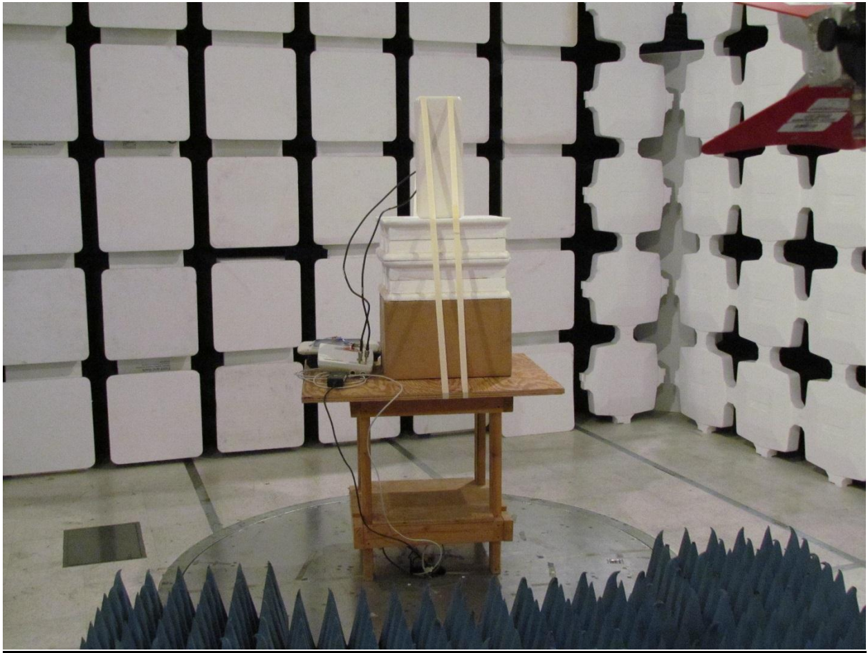
RDWN39 15.5 dBi ant Sector RW-9061-5002 TX Spur 1-18G Back
