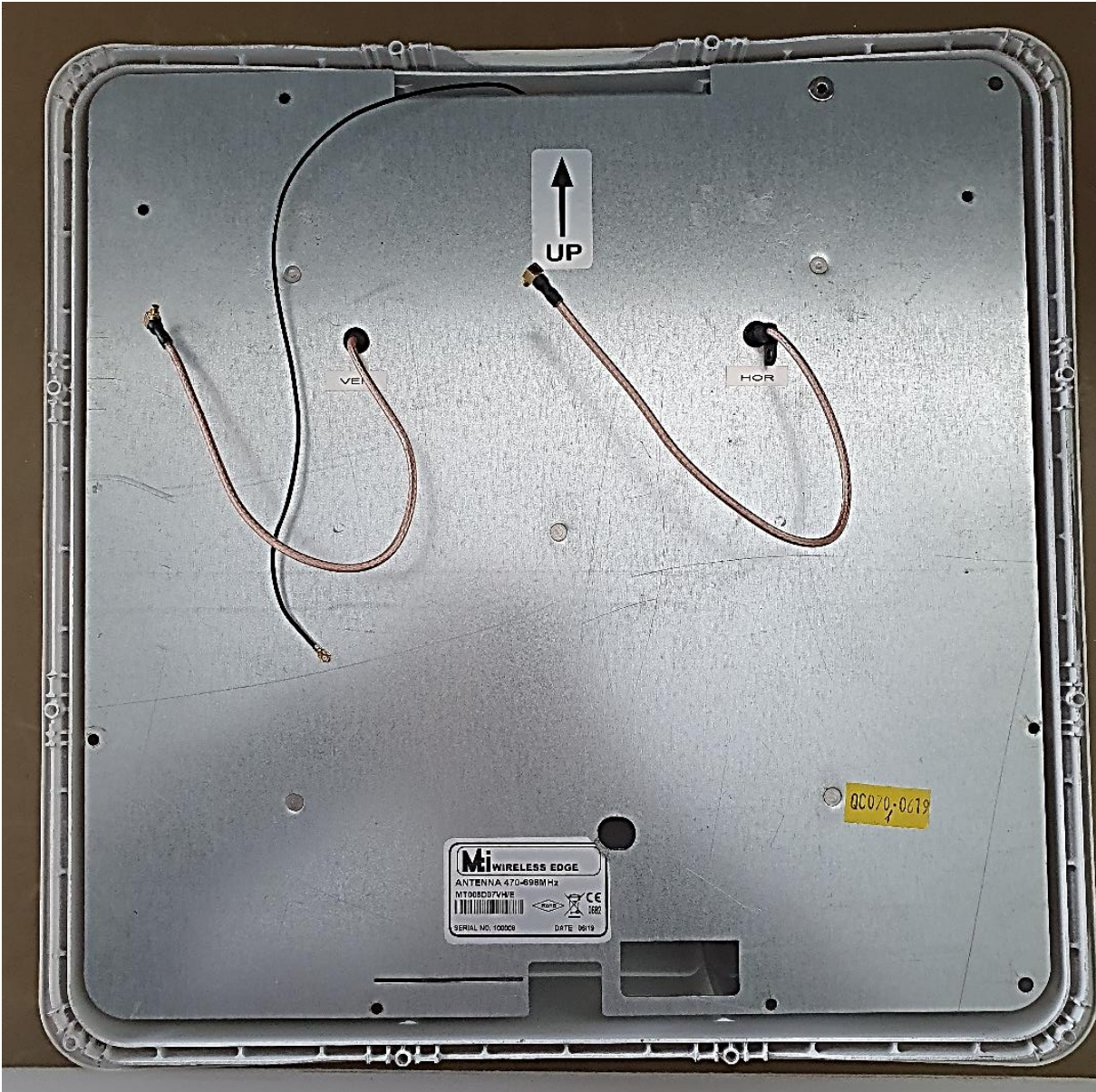
Photo 5: Antenna assembly top view
