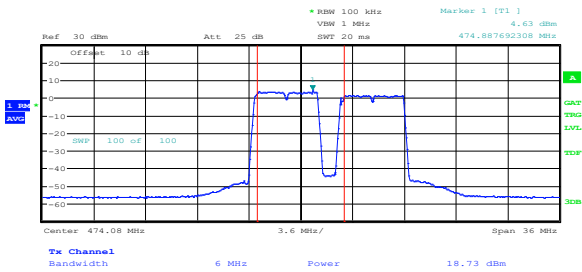
Figure 8.7-4: PSD within 100 kHz and Power within 6 MHz sample plot for multi 6 MHz channel
