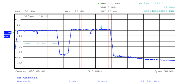
Figure 8.7-5: PSD within 100 kHz and Power within 6 MHz sample plot for multi 12 MHz channel
