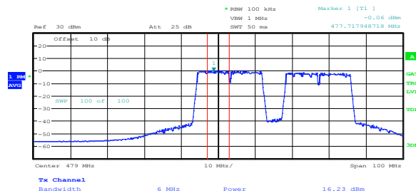
Figure 8.7-6: PSD within 100 kHz and Power within 6 MHz sample plot for multi 24 MHz channel
