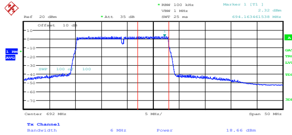
Figure 8.7-3: PSD within 100 kHz and Power within 6 MHz sample plot for single 24 MHz channel
