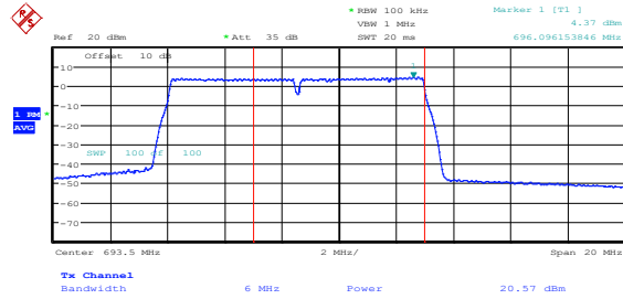
Figure 8.7-2: PSD within 100 kHz and Power within 6 MHz sample plot for single 12 MHz channel
