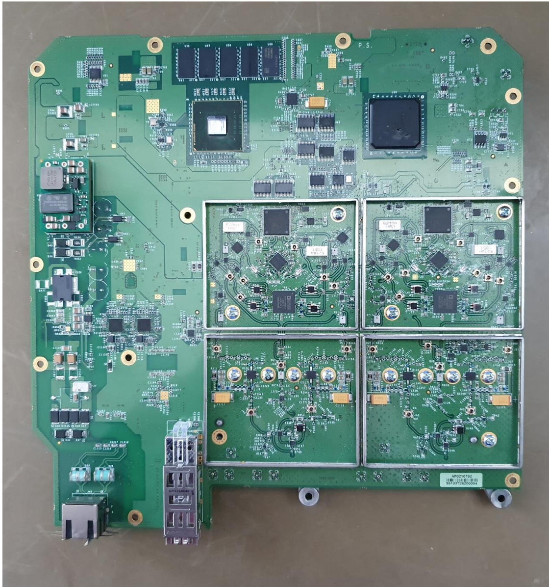
Photo 3: PCB P.S. view with shields off
