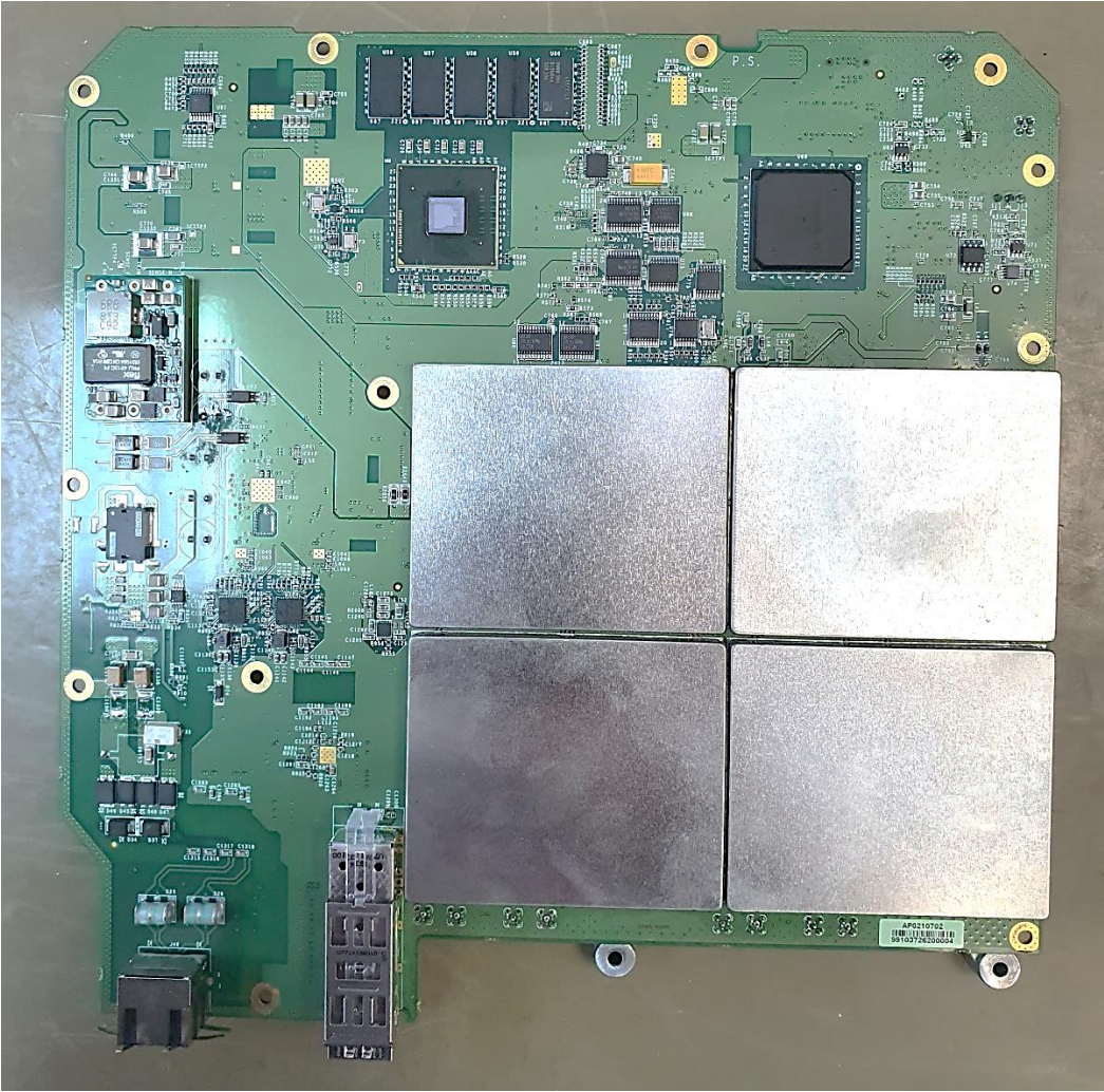
Photo 2: PCB P.S. view
