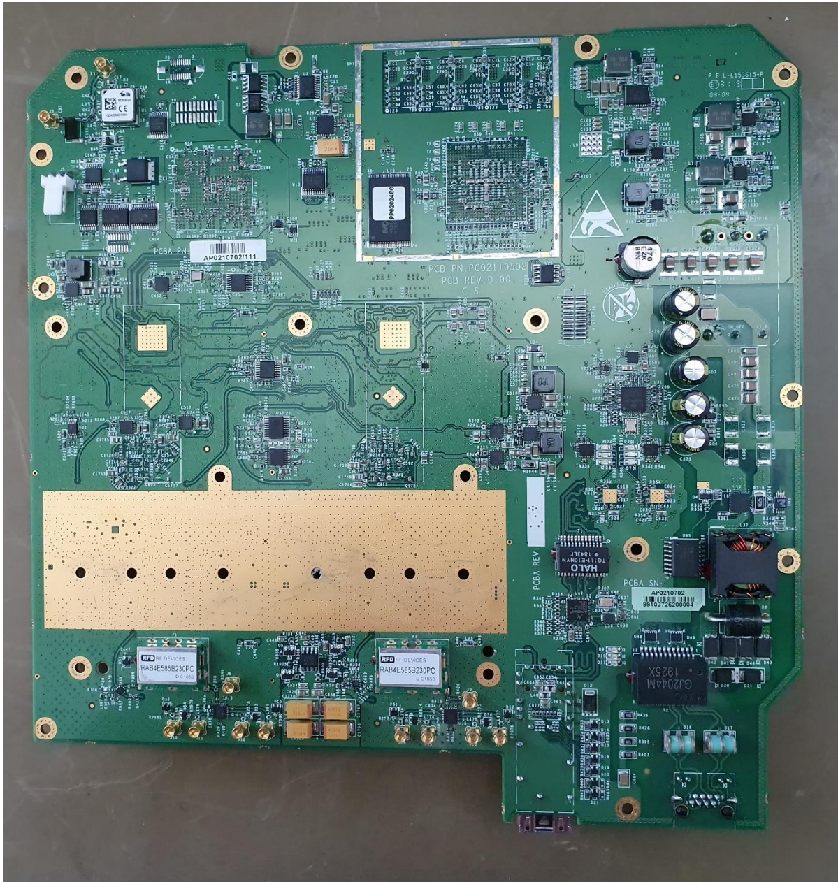
Photo 5: PCB C.S. view with heatsink off
