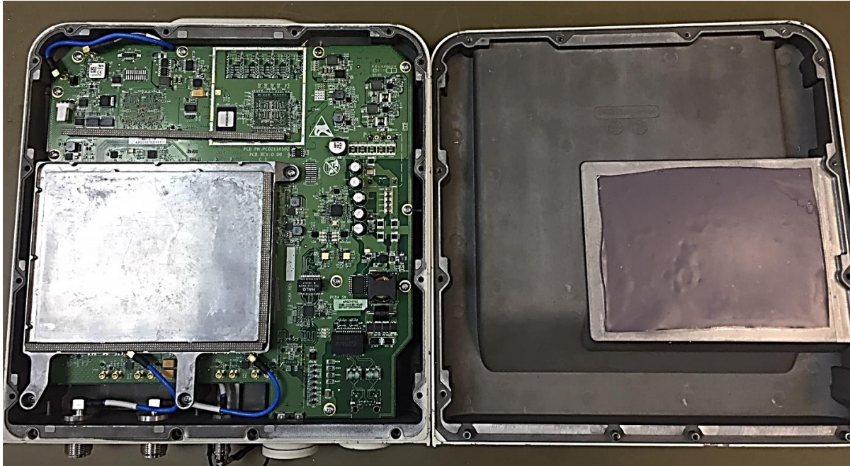
Photo 1: Internal Assembly View
