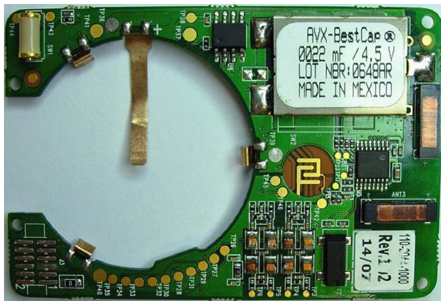
Figure 4 PCB Side 1
