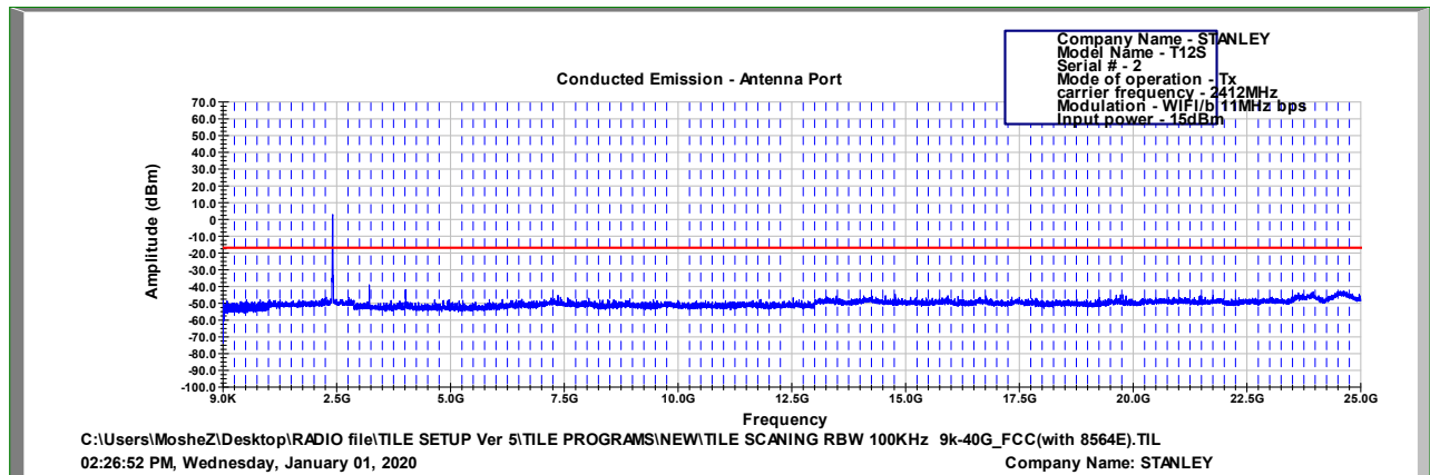
Figure 106 2412.0 MHz, WI-FI/b(11Mbit/s)
