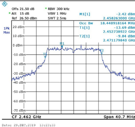
Figure 100. 2462.0 MHz, Wi-fi/n(65Mbit/s)
