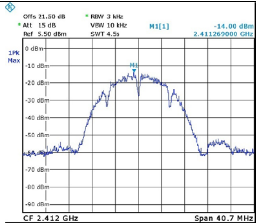
Figure 65. 2412.0 MHz, Wi-fi/b(1Mbit/s)
