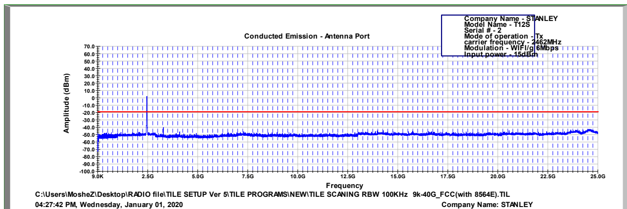
Figure 111 2462.0 MHz, WI-FI/g(6Mbit/s)
