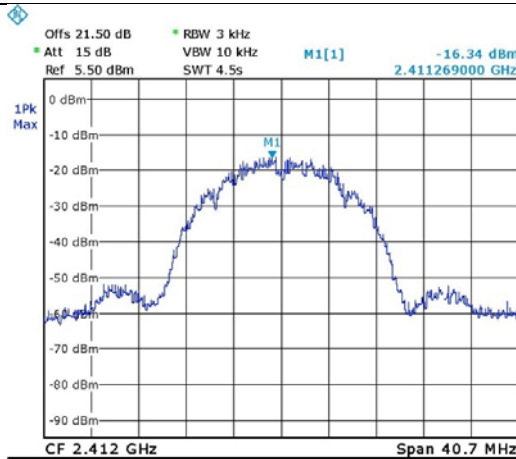
Figure 64. 2412.0 MHz, Wi-fi/b(11Mbit/s)
