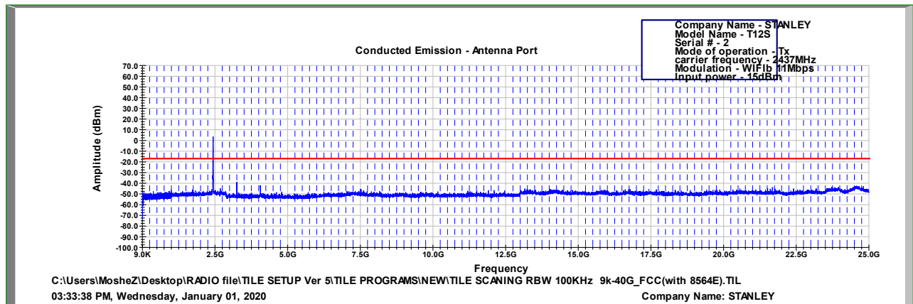
Figure 107 2437.0 MHz, WI-FI/b(11Mbit/s)
