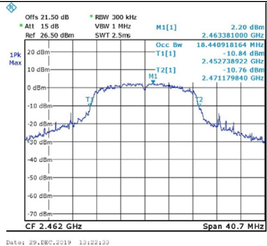
Figure 101. 2462.0 MHz, Wi-fi/n(6.5Mbit/s)
