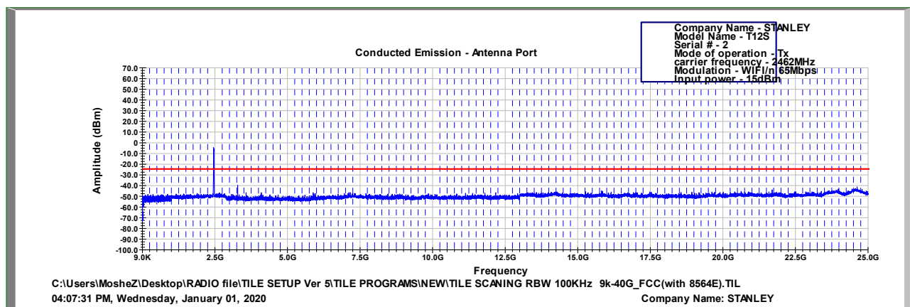
Figure 120 2462.0 MHz, WI-FI/n(65Mbit/s)
