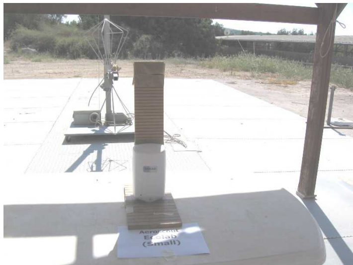
. Radiated Emission Test M/N: 92021184 (Ecolab NEXA small)
