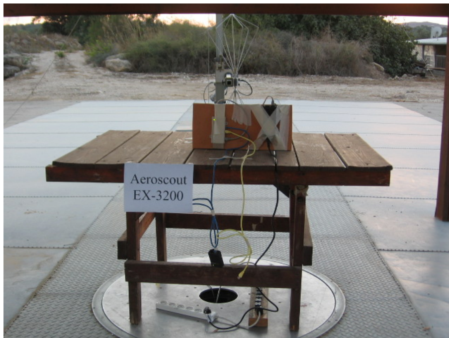
Figure 4. Radiated Emission Front
