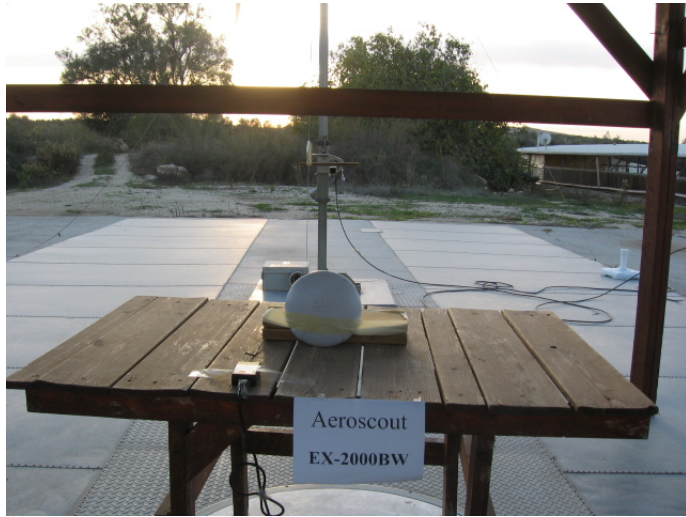
Radiated Emissions Tests Set-up
