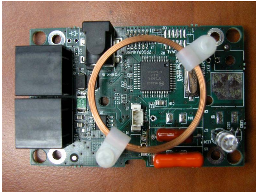
Figure 2 PCB Side 1
