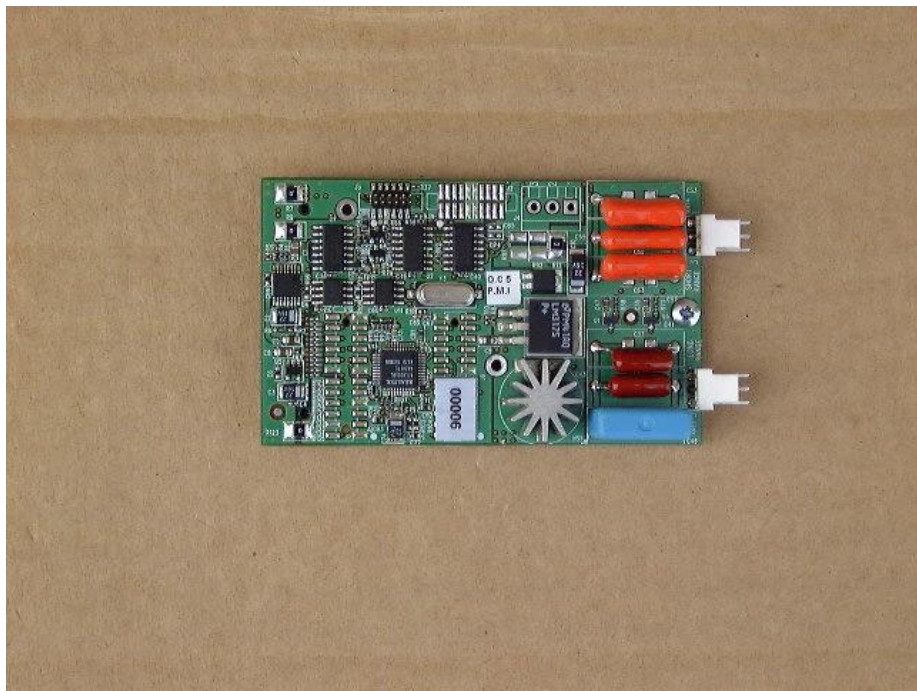
Figure 6 PCB 2 Side 1
