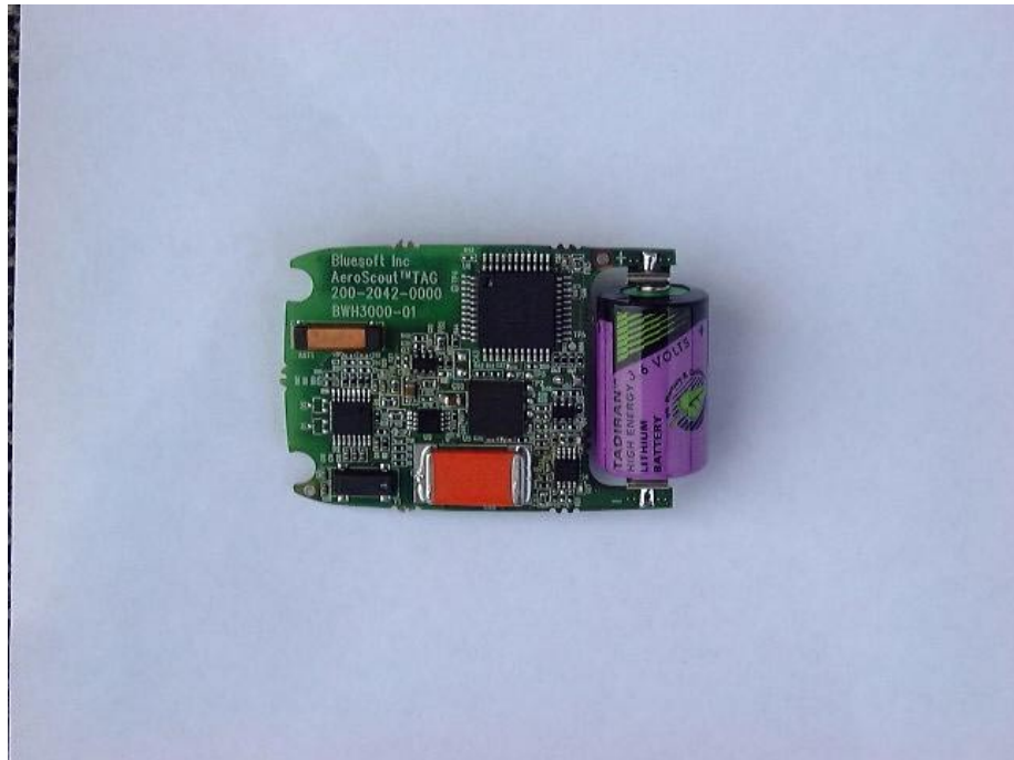
Figure 5 PCB Side 1 With Battery
