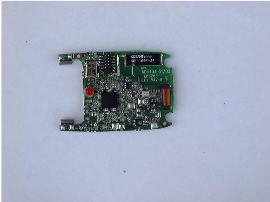
Figure 7 PCB Side 2
