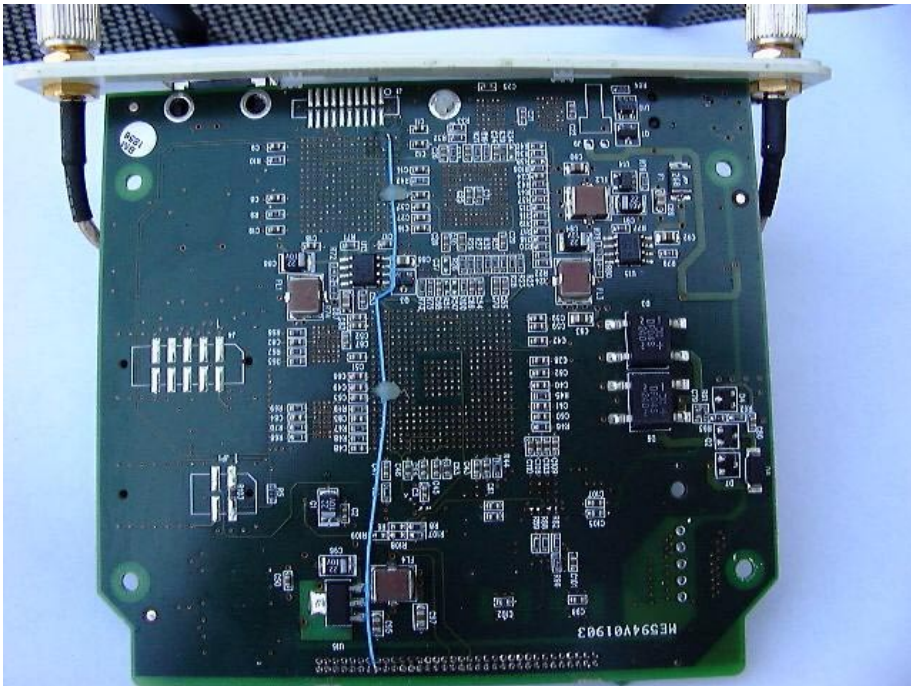
Figure 8 PCB Side 2
