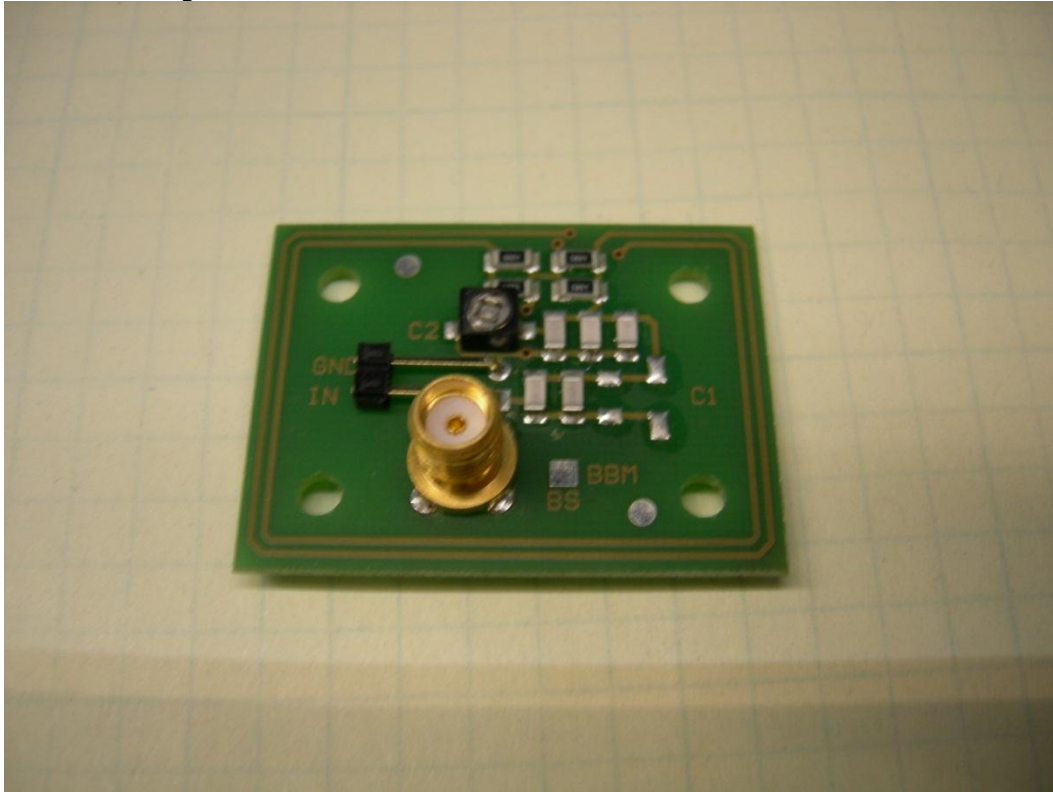
Small Rectangle Antenna
