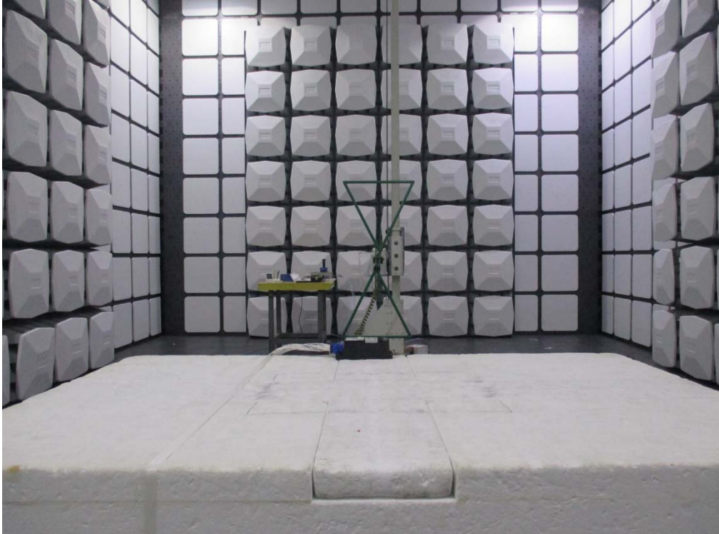
Description: Back View of Radiated Spurious Emission Test Setup (below 1GHz)
