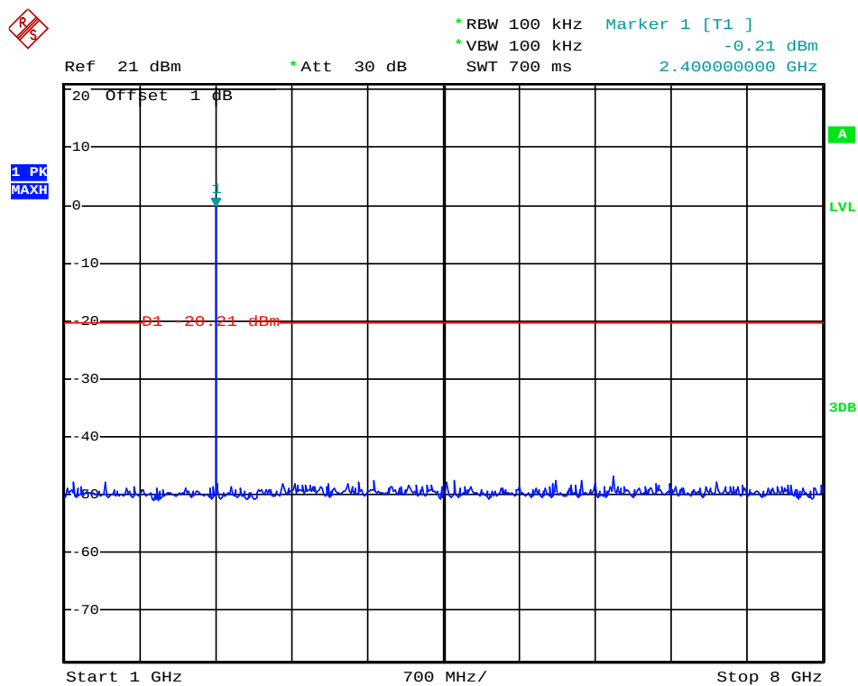
(Plot 4.9.3.A1: Channel 00: 2402MHz @ \pi/4 DQPSK)
