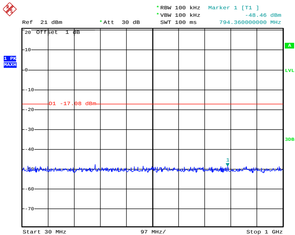
(Plot 4.9.2.B4: Channel 39: 2441MHz @ 8DPSK)
