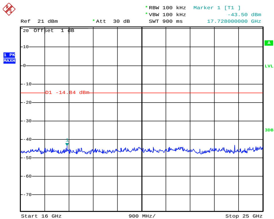
(Plot 4.9.1.B3: Channel 39: 2441MHz @ GFSK)
