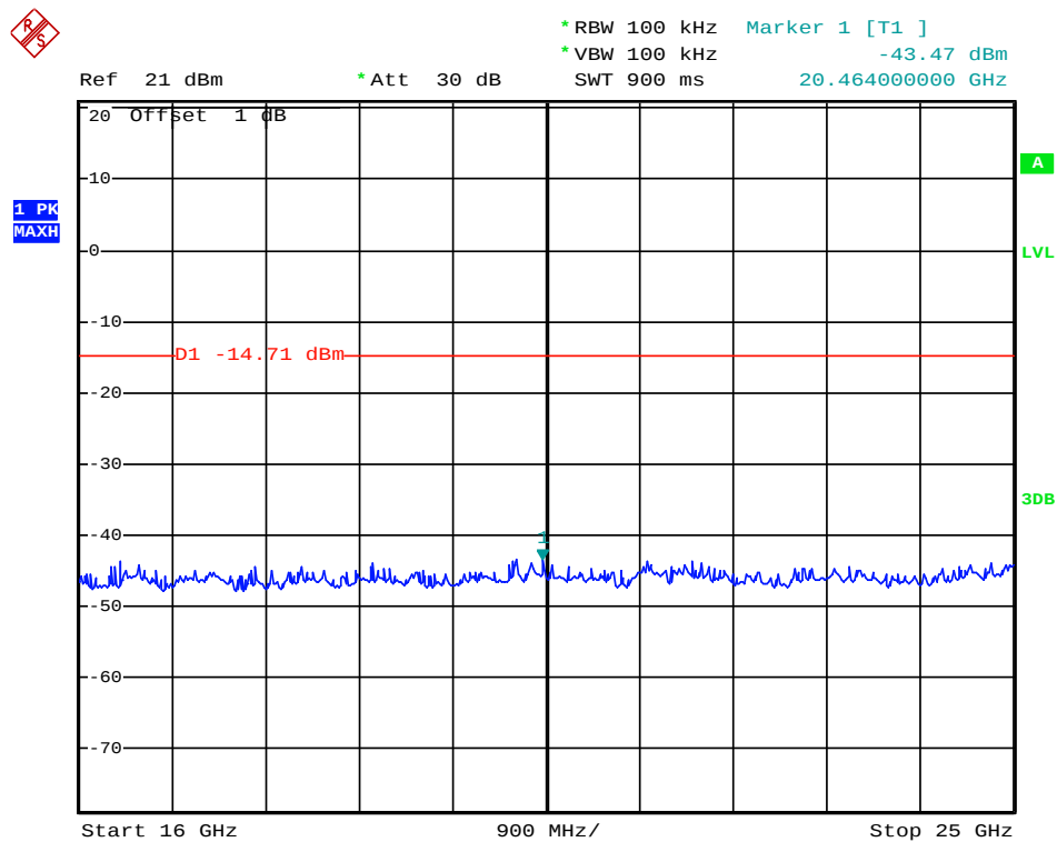
(Plot 4.9.1.C3: Channel 78: 2480MHz @ GFSK)
