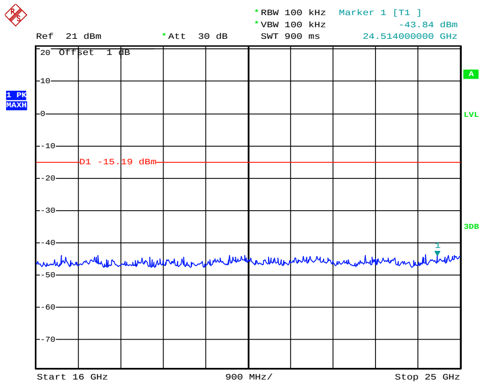
(Plot 4.9.3.C3: Channel 78: 2480MHz @ \pi/4 DQPSK)
