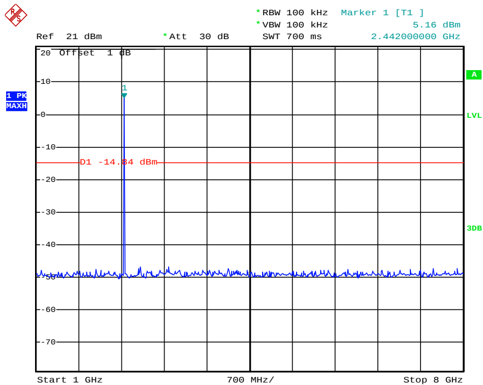
(Plot 4.9.1.B1: Channel 39: 2441MHz @ GFSK)
