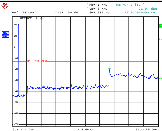
1GHz~20GHz
