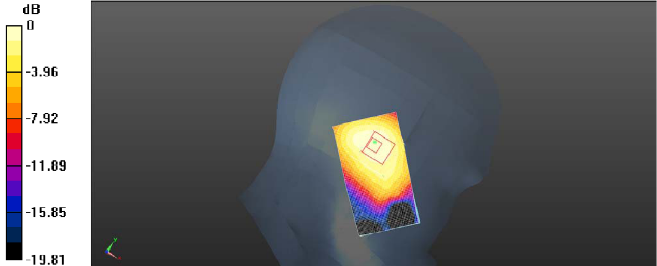
Plot 24: Left Head Touch (GSM1900 GPRS 4TS High Channel)
