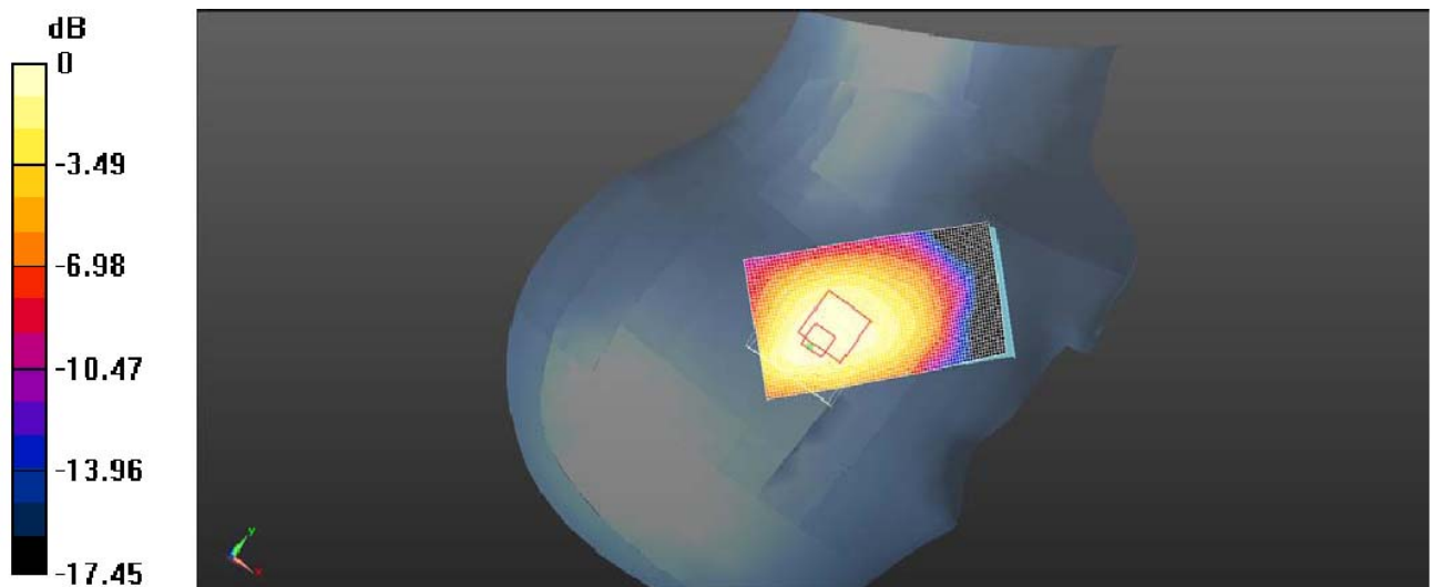
Plot 29: Right Head Touch (GSM1900 Middle Channel)
