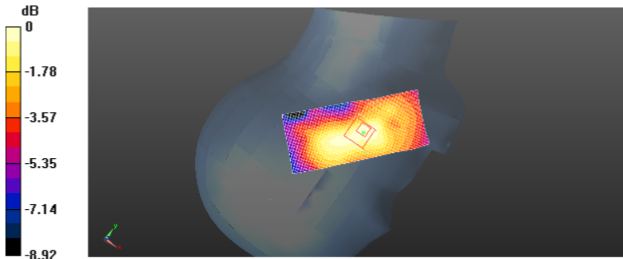
Plot 46: Right Head Tilt (WiFi-Middle Channel-Channel 6-2437MHz)
