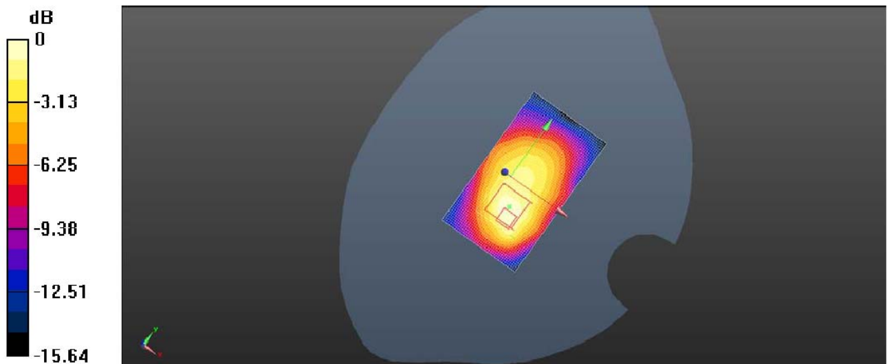
Plot 40: Body Top side (GSM1900 GPRS 4TS Middle Channel)
