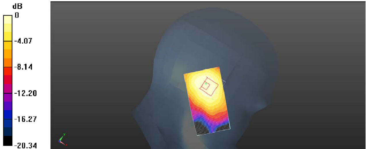
Plot 23: Left Head Touch (GSM1900 Middle Channel)
