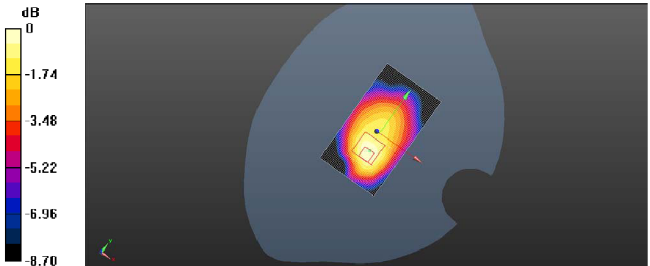
Plot 41: Body Rear (GSM1900 EGPRS 4TS Middle Channel)
