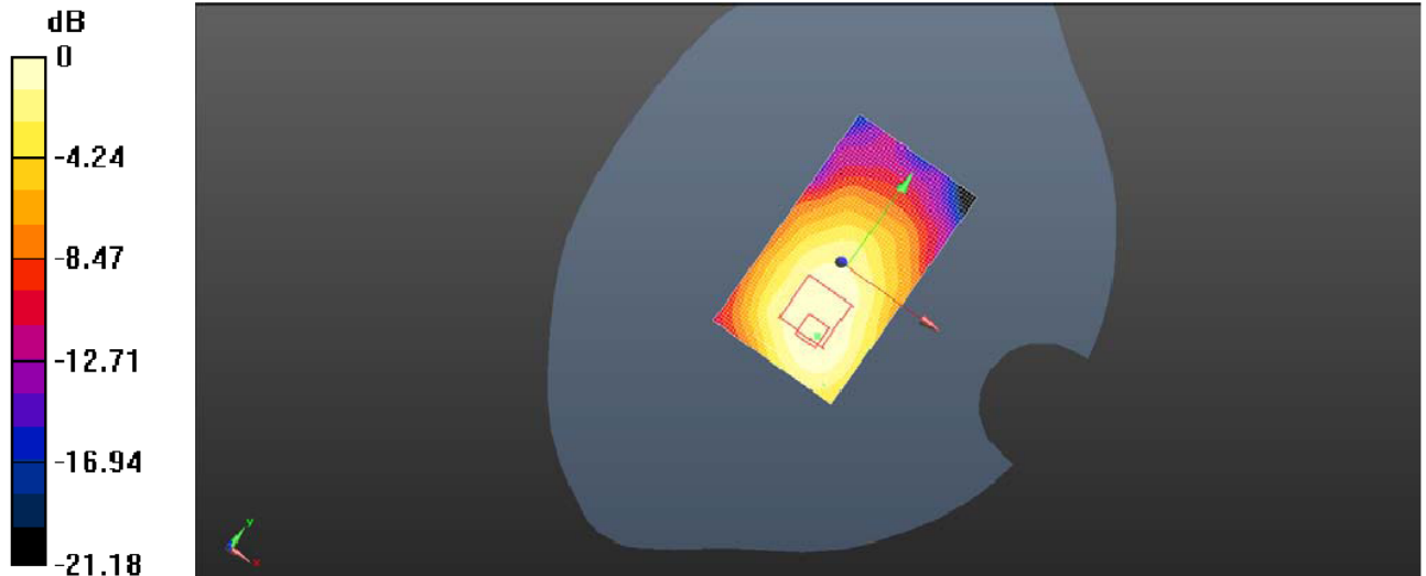
Plot 34: Body Front (GSM1900 GPRS 4TS Middle Channel)
