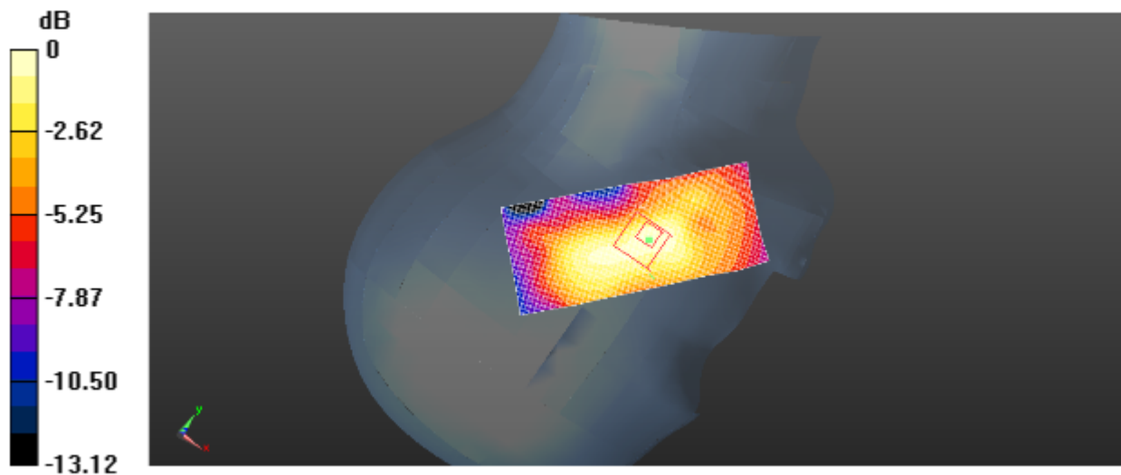
Plot 45: Right Head Touch (WiFi-Middle Channel-Channel 6-2437MHz)
