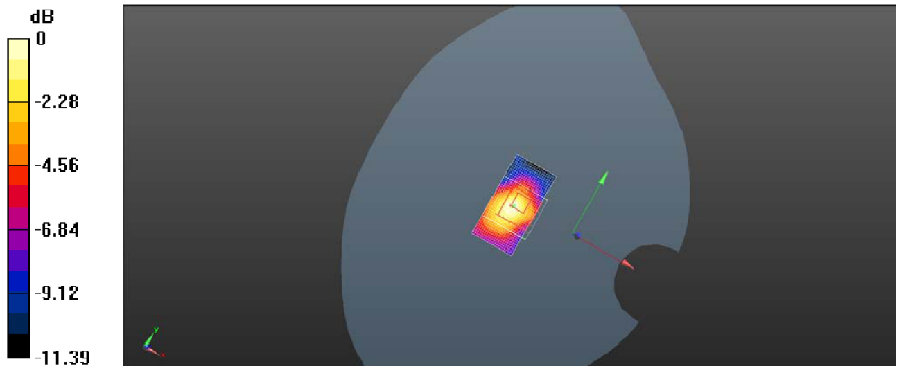
Plot 19: Body Top Side (GSM850 GPRS 4TS Middle Channel)
