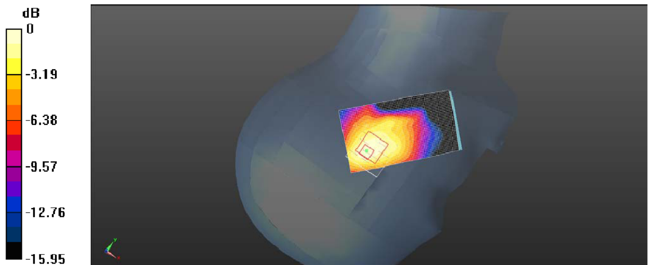
Plot 9: Right Head Touch (GSM850 High Channel)
