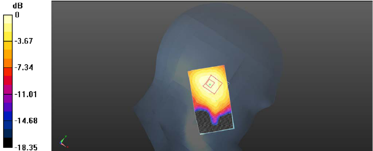
Plot 22: Left Head Touch (GSM1900 Low Channel)
