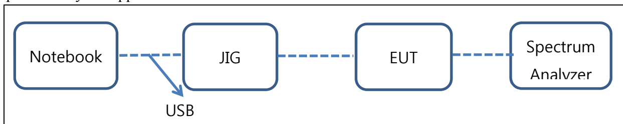
[System Block Diagram of Test Configuration]
