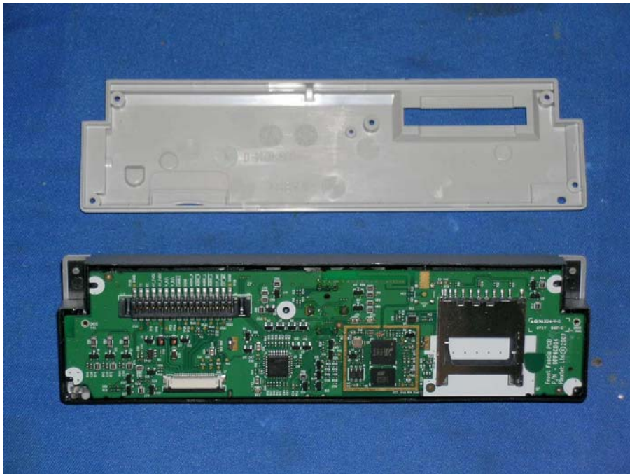
Control Stereo Panel assembly
