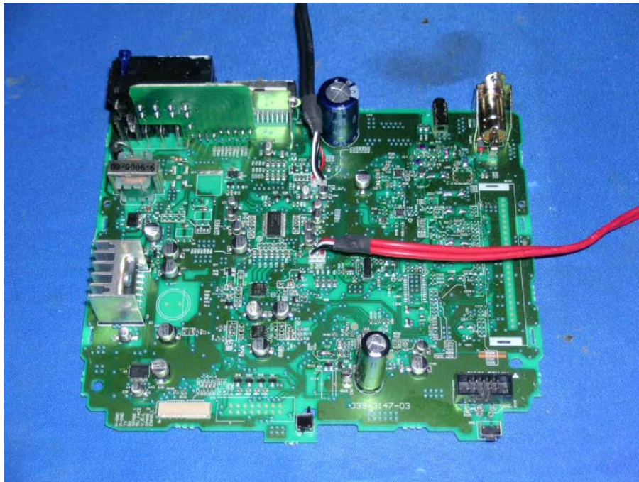
Car Stereo Main PCB comp side
