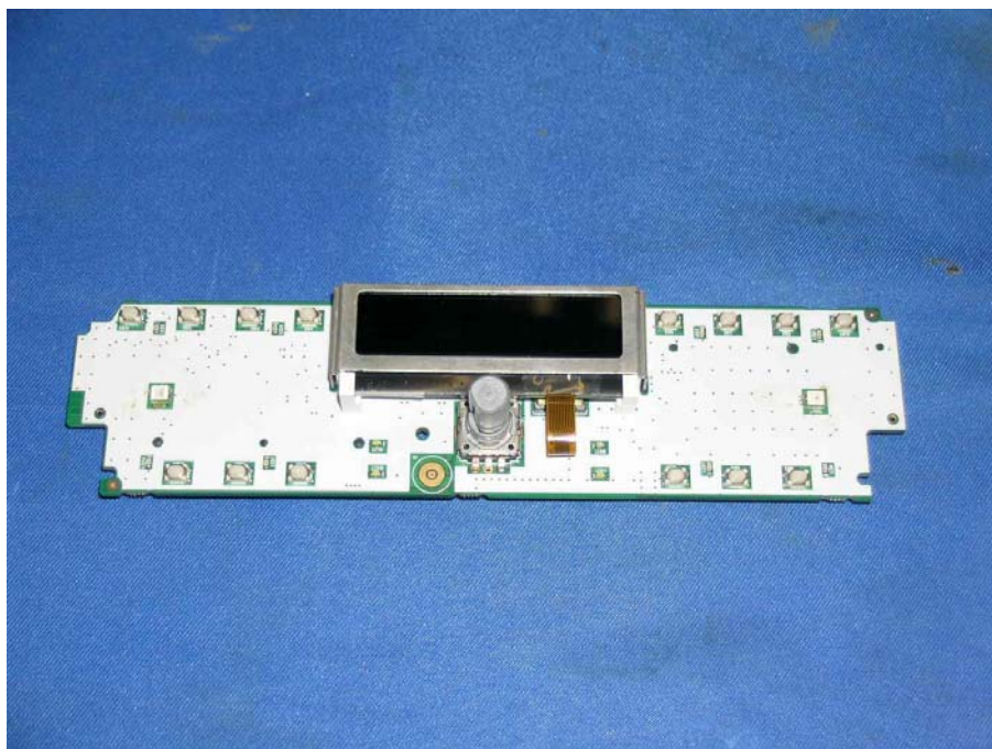
Control Stereo Panel Main PCB solder side (View 1)
