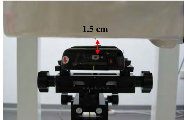
Fig.8 EUT back REID to flat phantom
