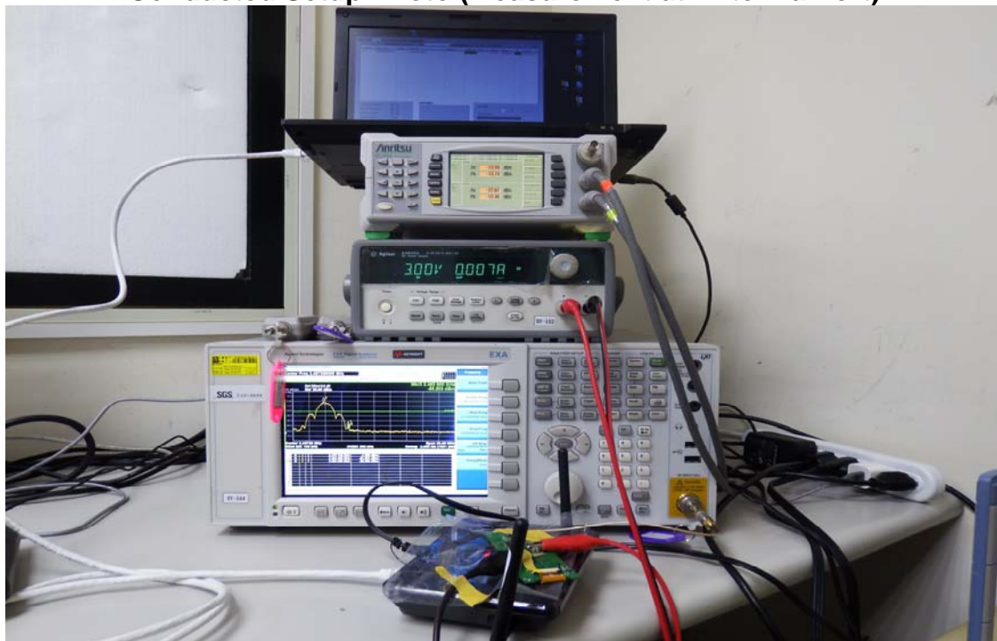
Conducted Setup Photo (Measurement at Antenna Port)
