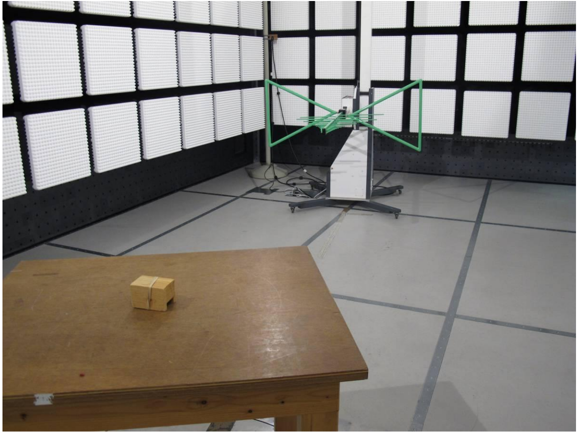
Photograph 2: Test setup radiated emissions (30 - 1000 MHz)
