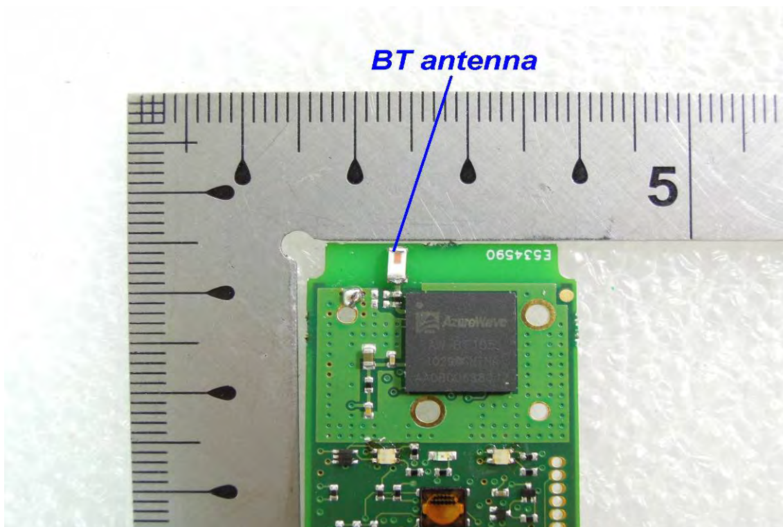
BT Antenna
