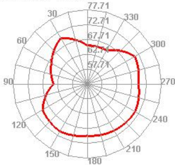
Wifi 165 TIS H
