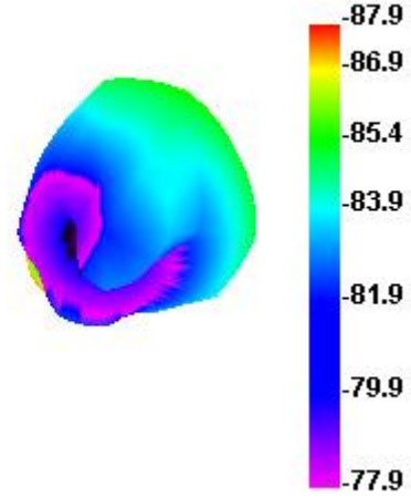
Wifi 6 TIS
