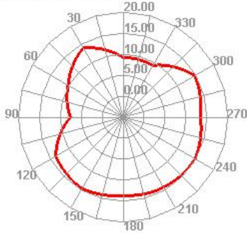
Wifi 165 TRP H
