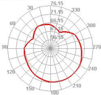
Wifi 36 TIS H
