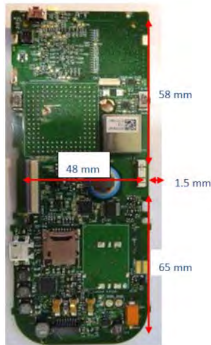
Fig.9 Antenna position of EUT (Back view)
