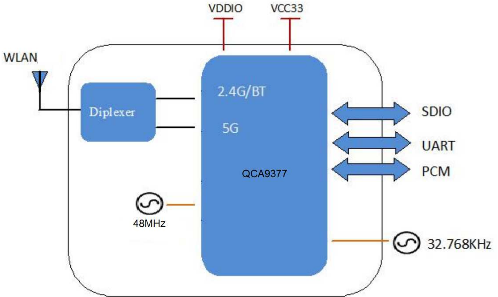
8223A WiFi Module Block Diagram
