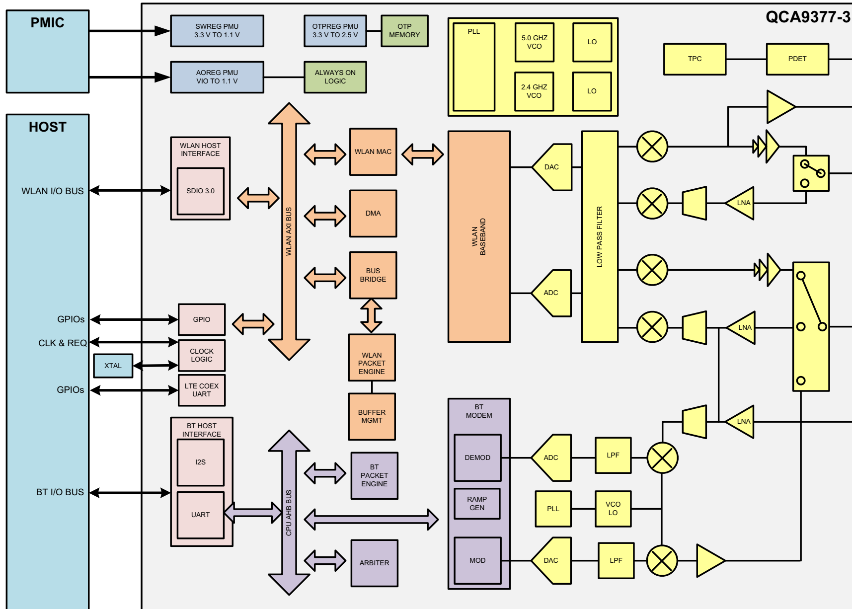
Figure 1-1 QCA9377-3 functional block diagram
