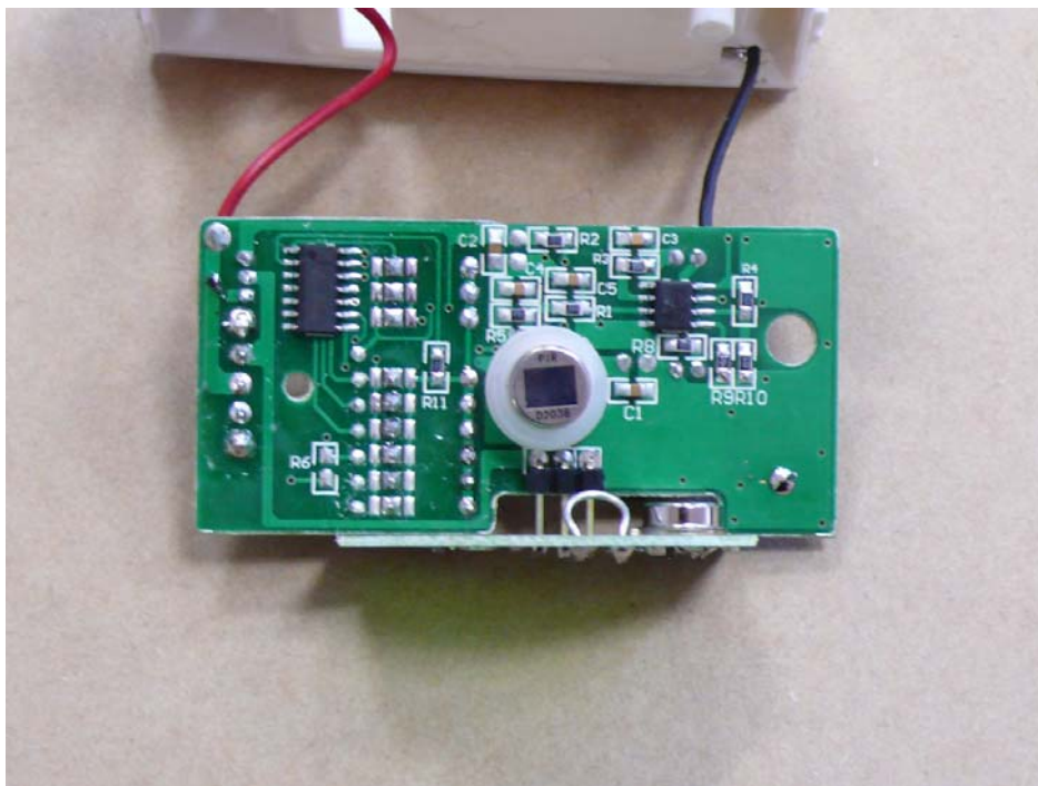
Back side of PCB1
