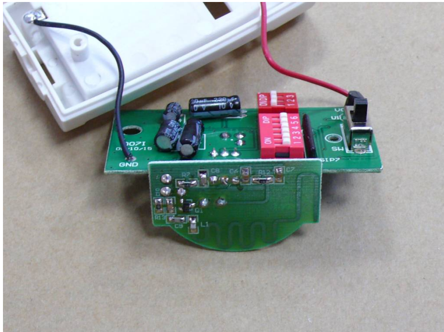
Front side of PCB2
