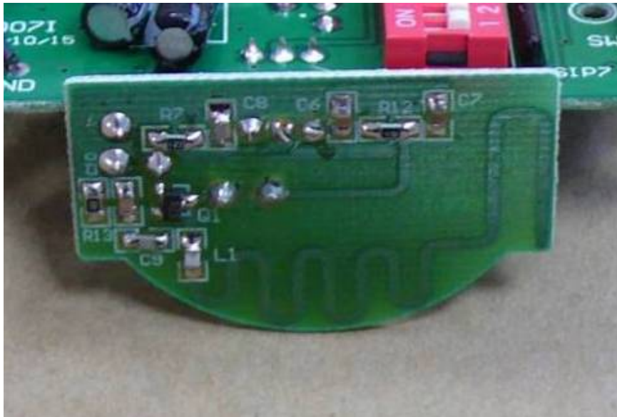
Front side of PCB2
