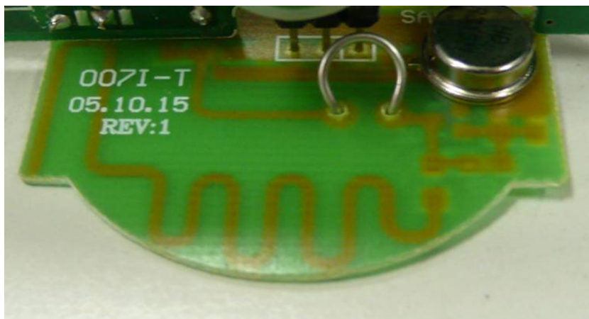
Back side of PCB2
