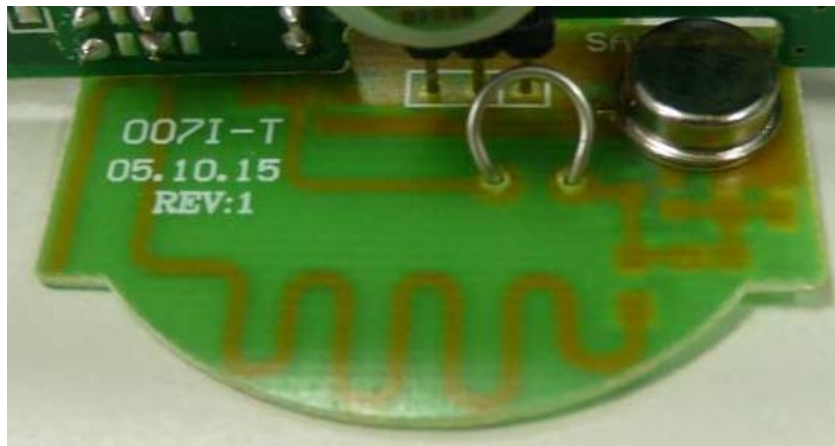
Back side of PCB2
