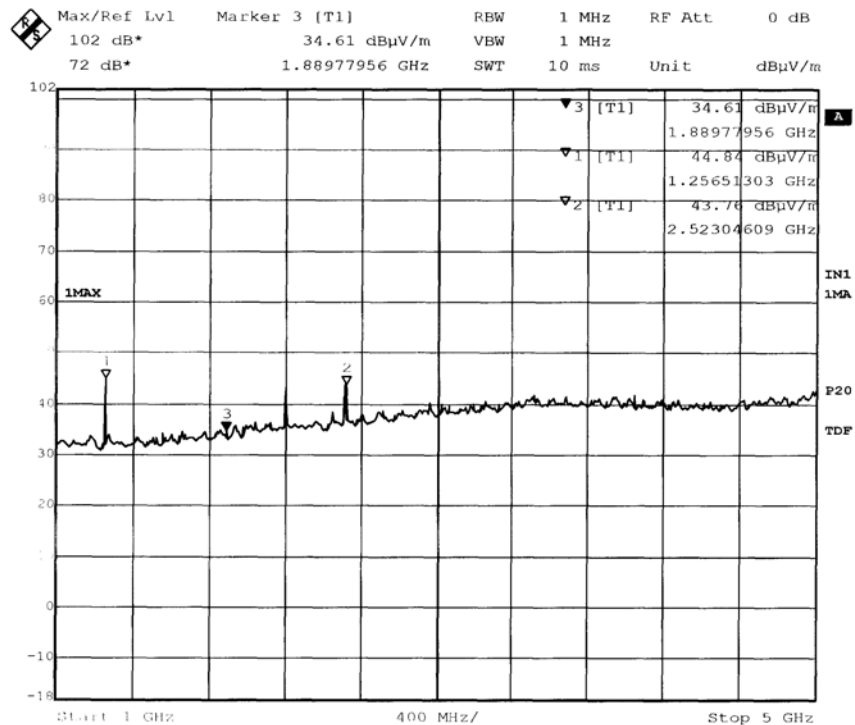
Transmission (Vertical)
