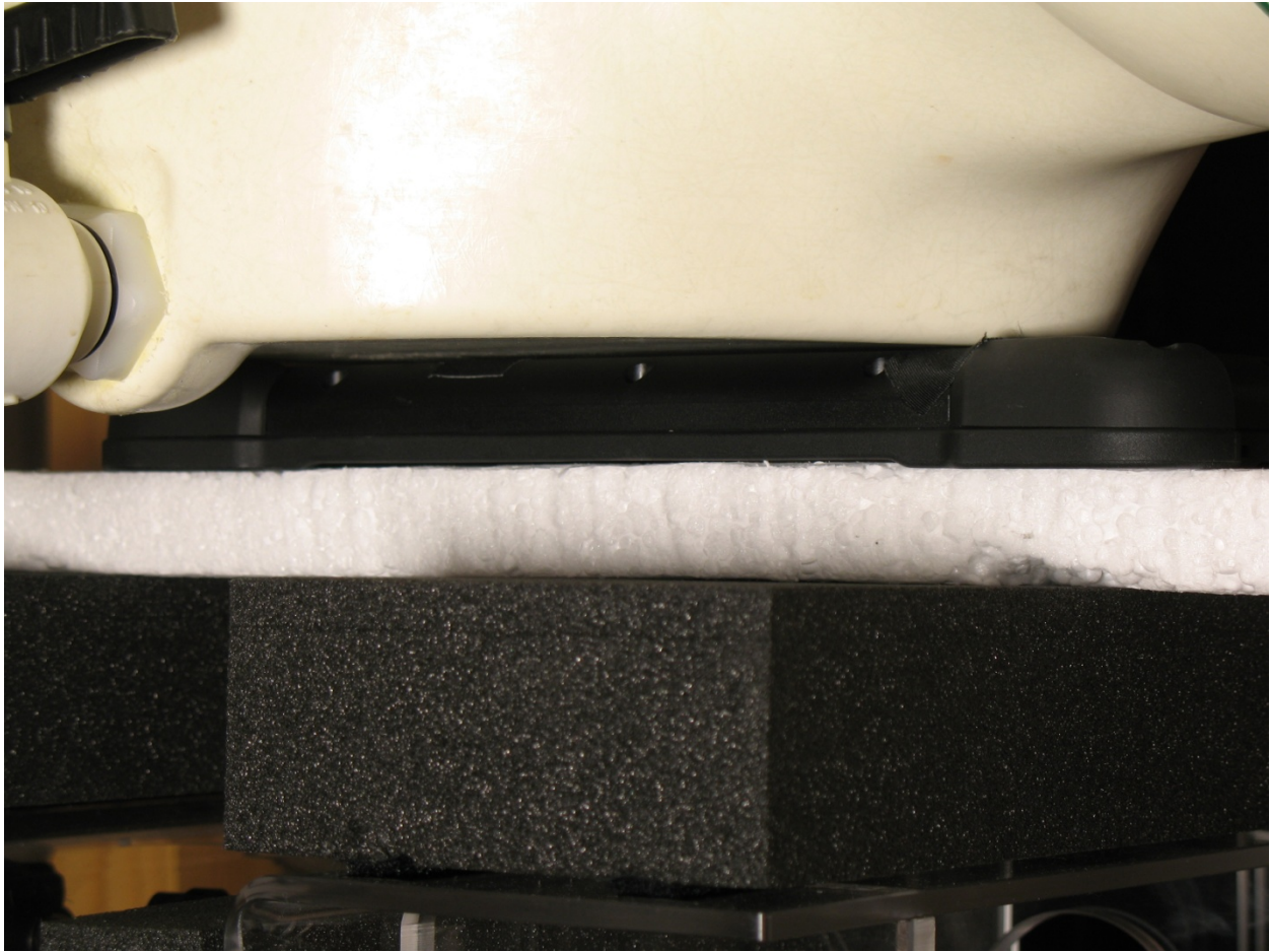
Figure 1: Device Positioning for SAR Scans – Lap Position – Back Against Phantom
