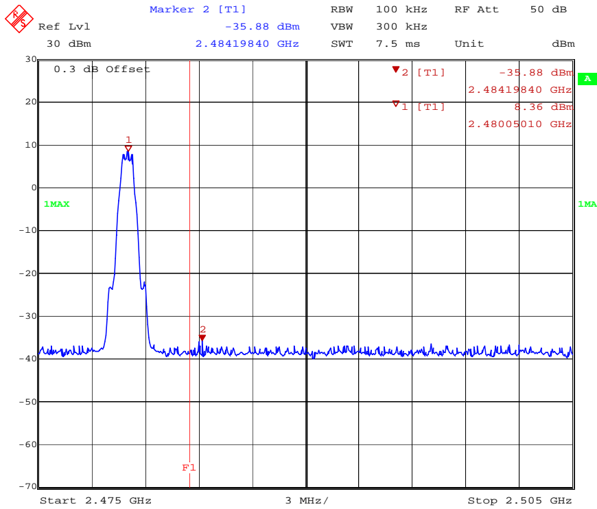
High Band Edge Plot, High Channel
