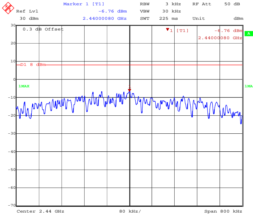
PSD Middle Channel
