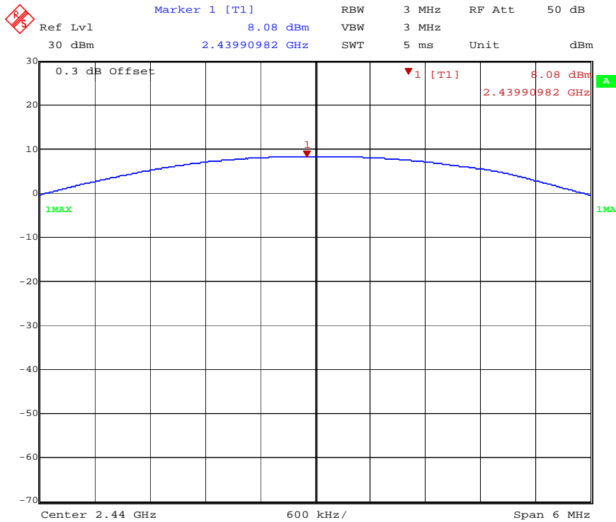
Peak Output Power, Mid Channel
