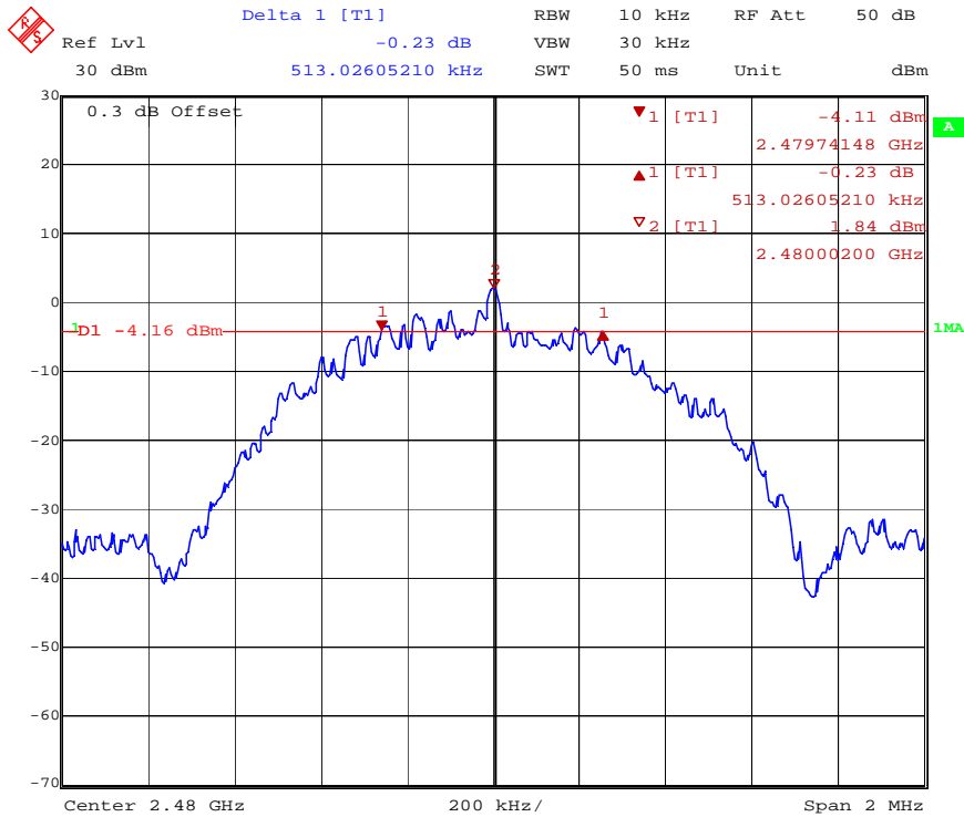
6dB Bandwidth, High Channel
