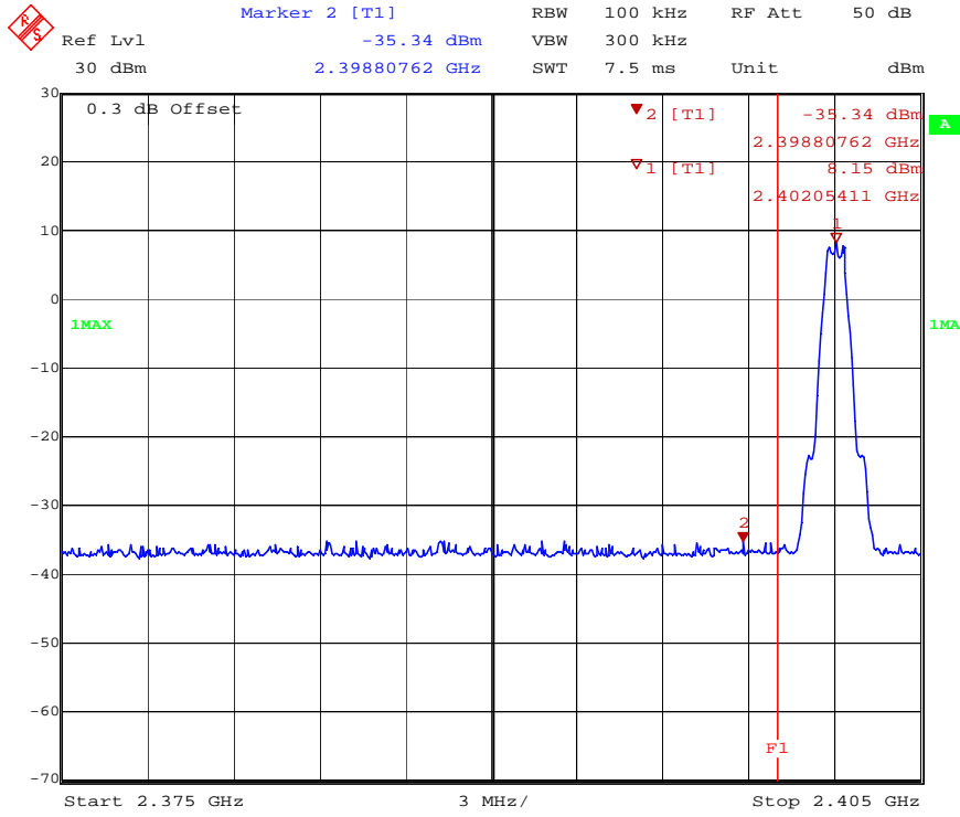
Low Band Edge Plot, Low Channel
