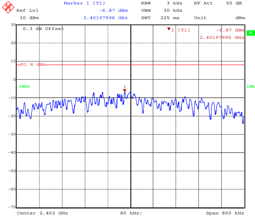
PSD Low Channel
