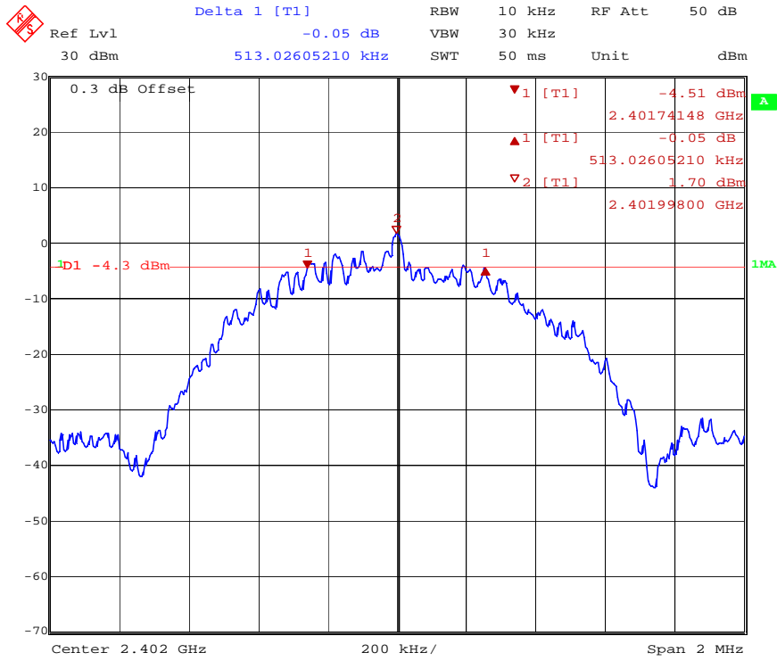
6dB Bandwidth, Low Channel
