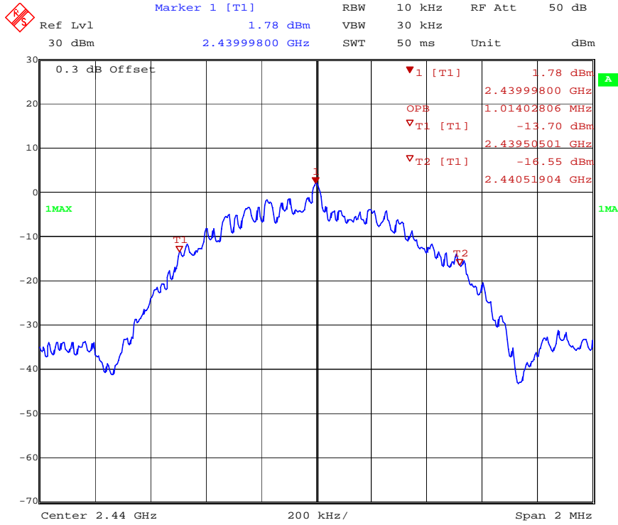
99% Bandwidth, Middle Channel
