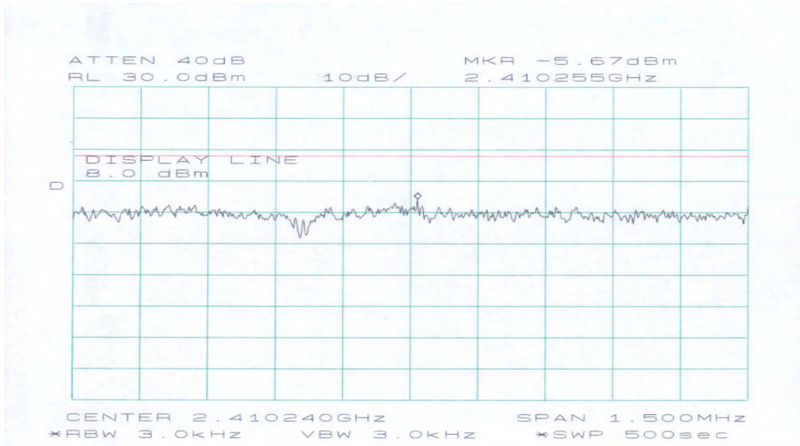
Peak Power Spectral Density for 2410 MHz (Low channel)
