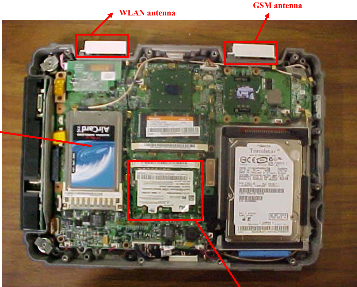
EUT – Internal view showing GSM & WLAN modules
