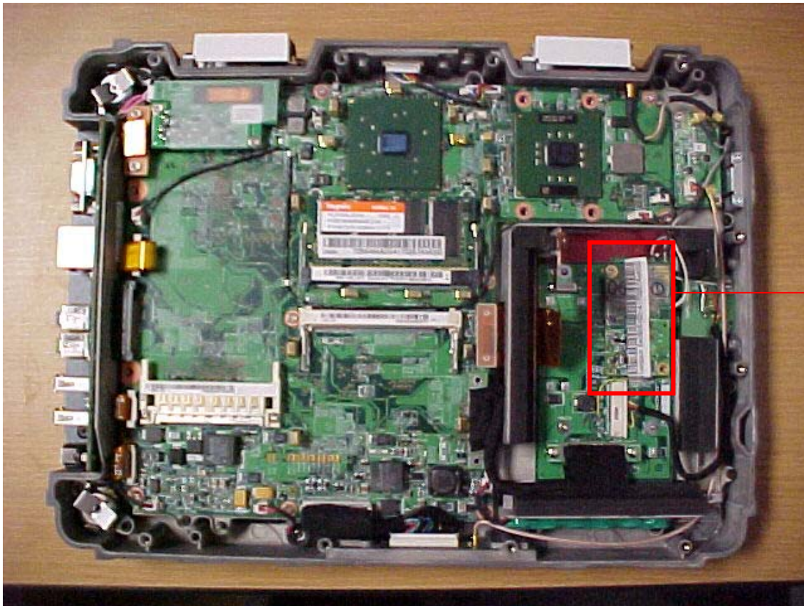
EUT – Internal view showing BT radio module
