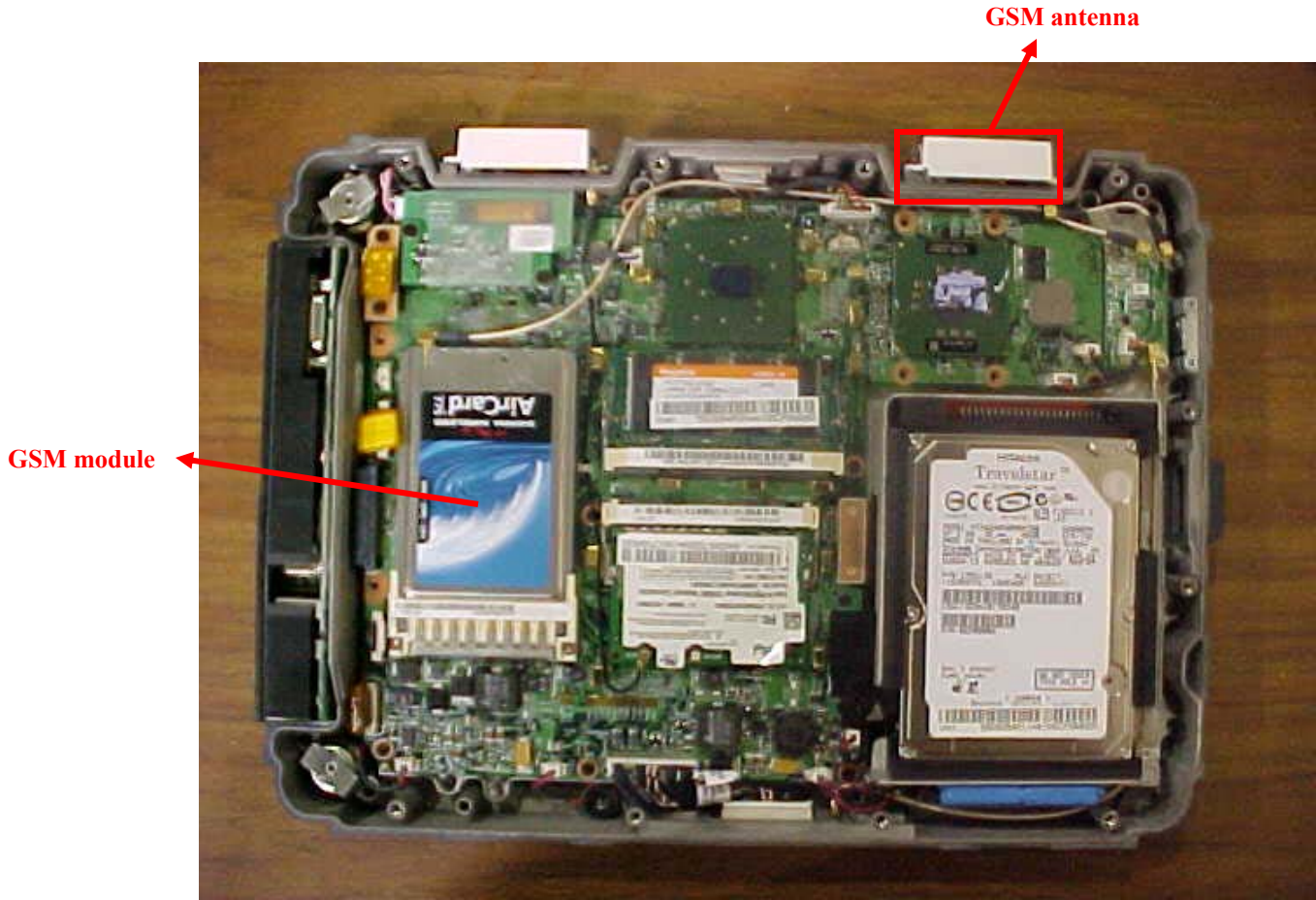
EUT – Internal view showing GSM module
