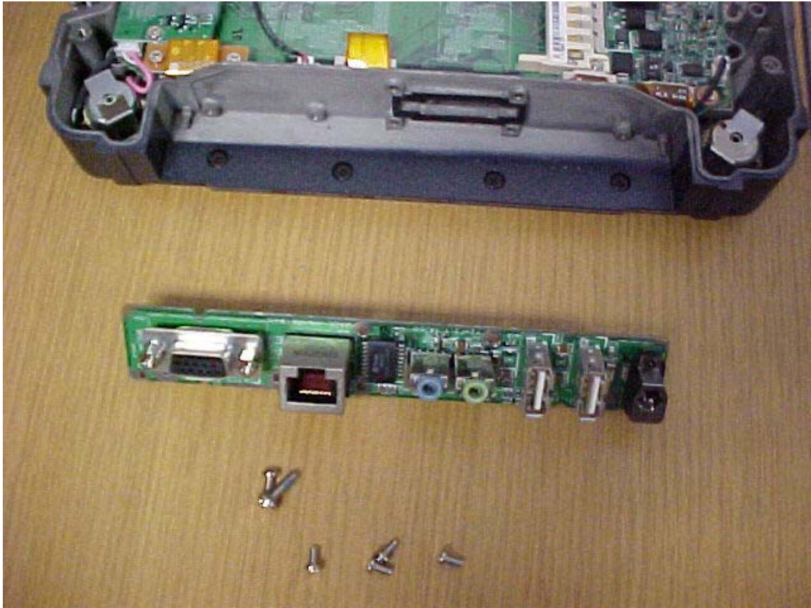
I/O Ports
