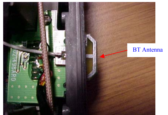
EUT – Internal view showing BT & CDMA module
