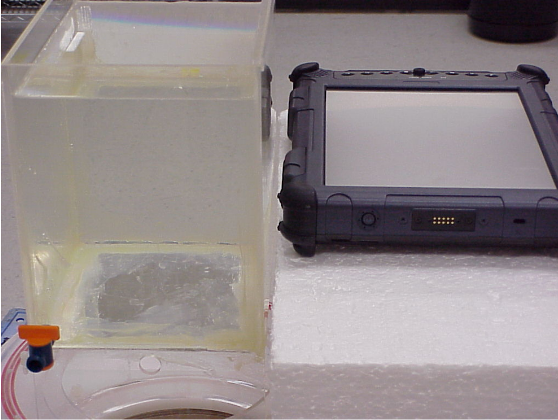
Photo 4. GPRS antenna bystander position
