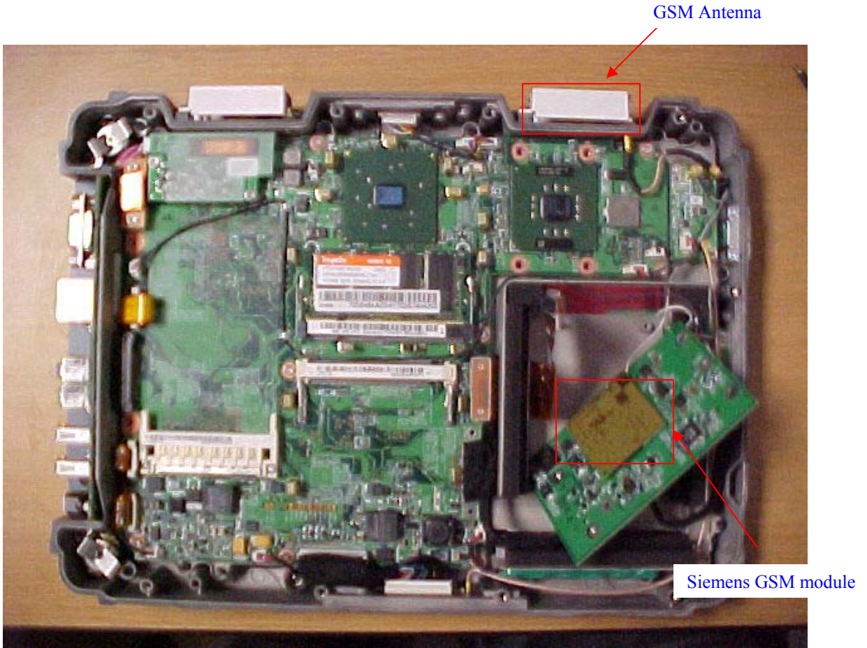
EUT – Internal view showing GSM module
