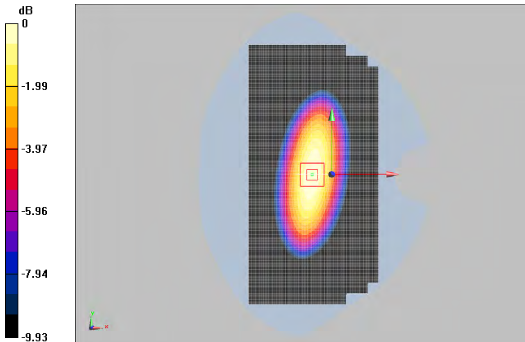
0 dB = 2.35W/kg
