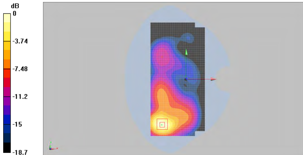
0 dB = 0.848W/Kg
