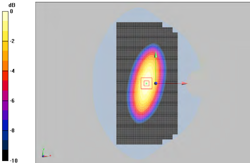
0 dB = 2.30W/kg
