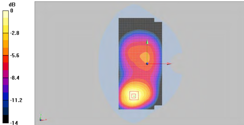
0 dB = 0.466W/Kg
