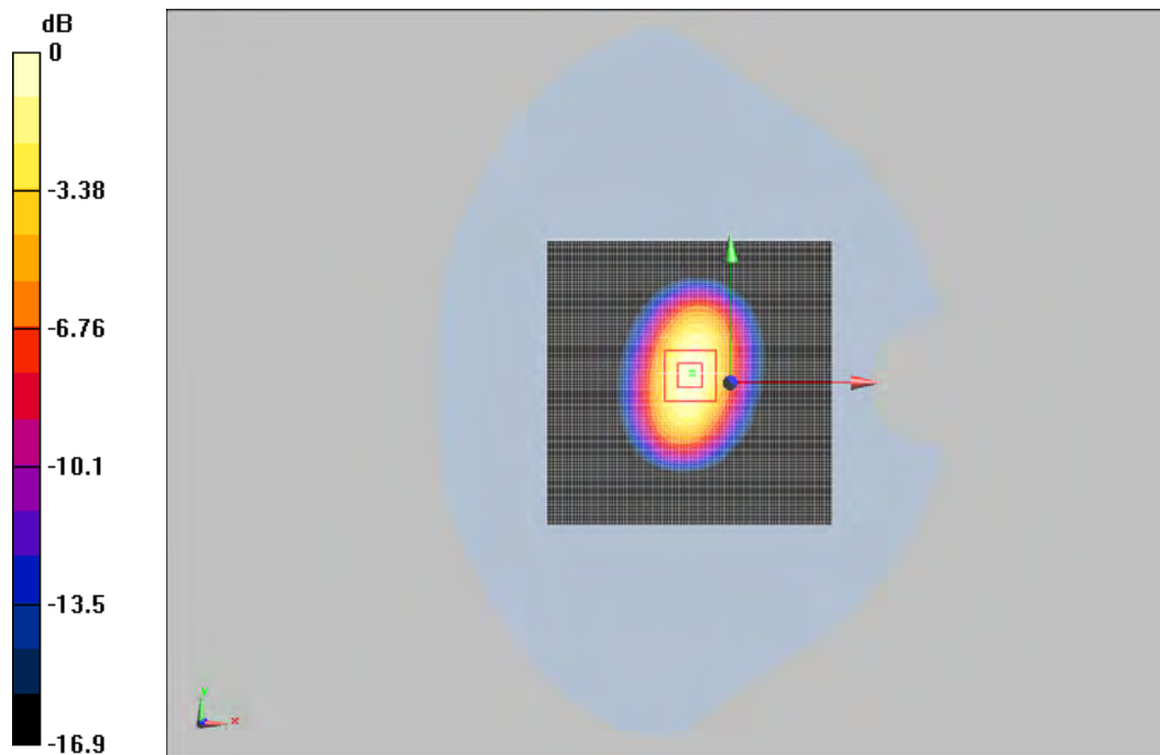
0 dB = 10.9W/kg
