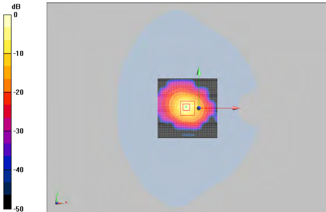
0 dB = 41.7W/kg
