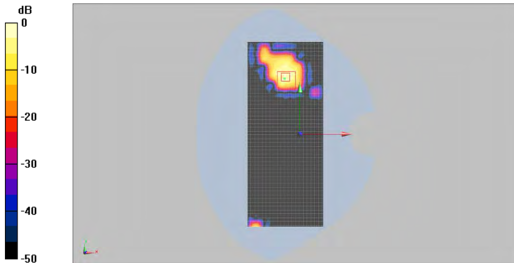
0 dB = 0.116W/Kg
