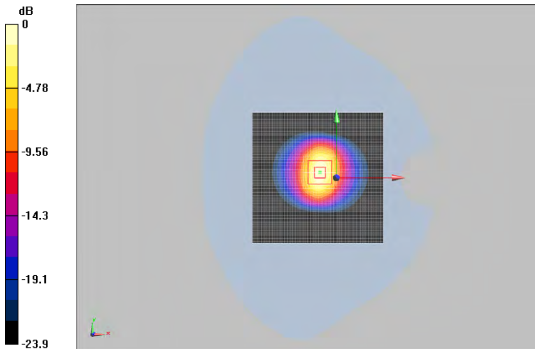
0 dB = 15.9W/kg
