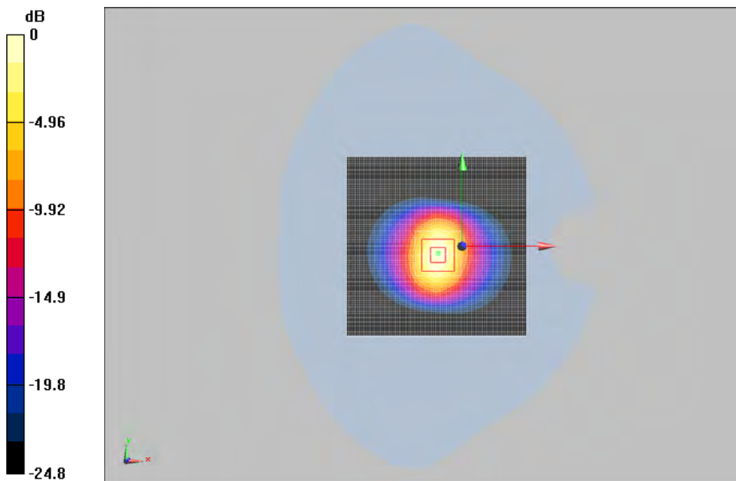
0 dB = 16W/kg
