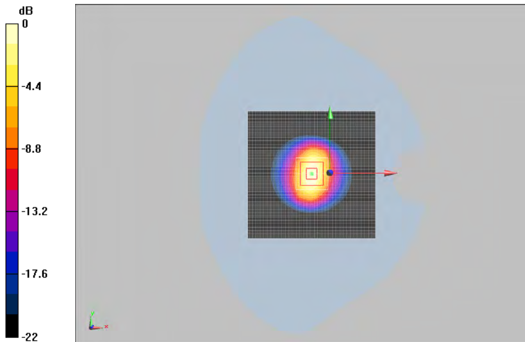
0 dB = 14.6W/kg
