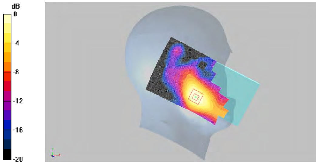
0 dB = 0.168W/Kg
