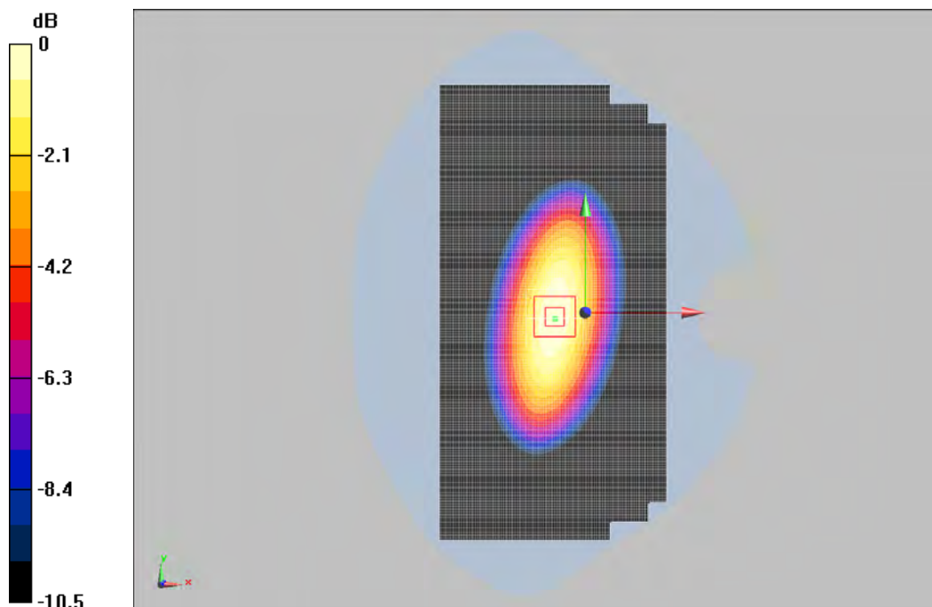
0 dB = 2.67W/kg
