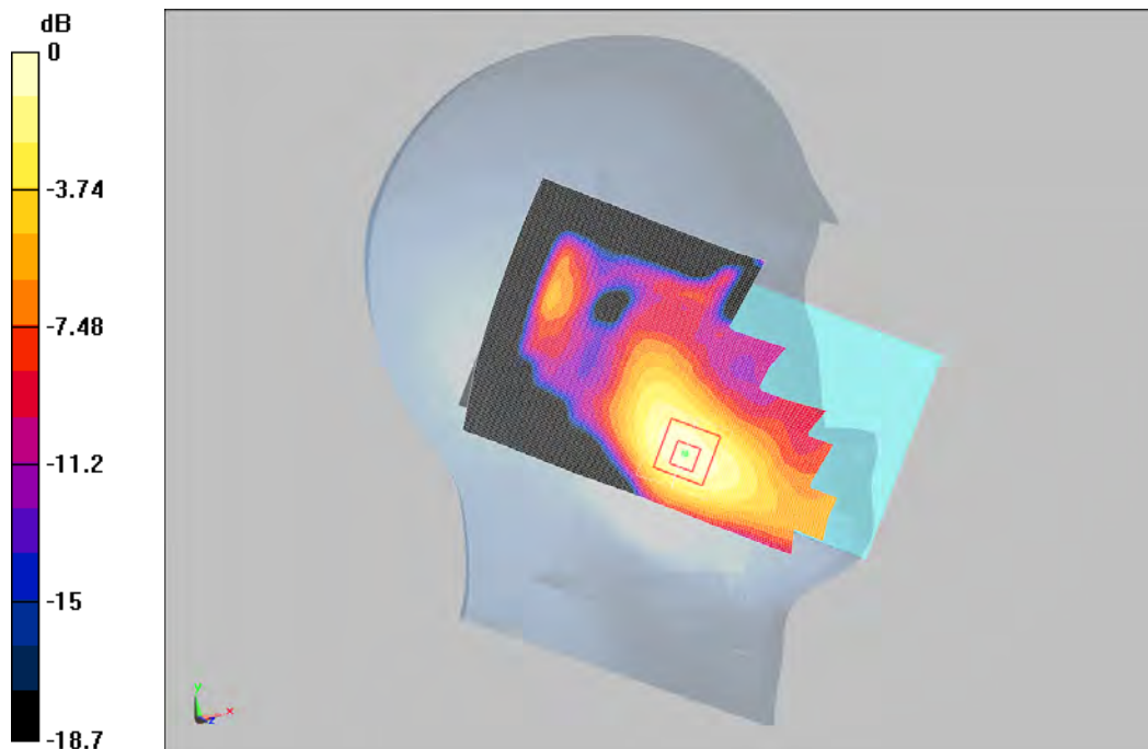
0 dB = 0.079W/kg
