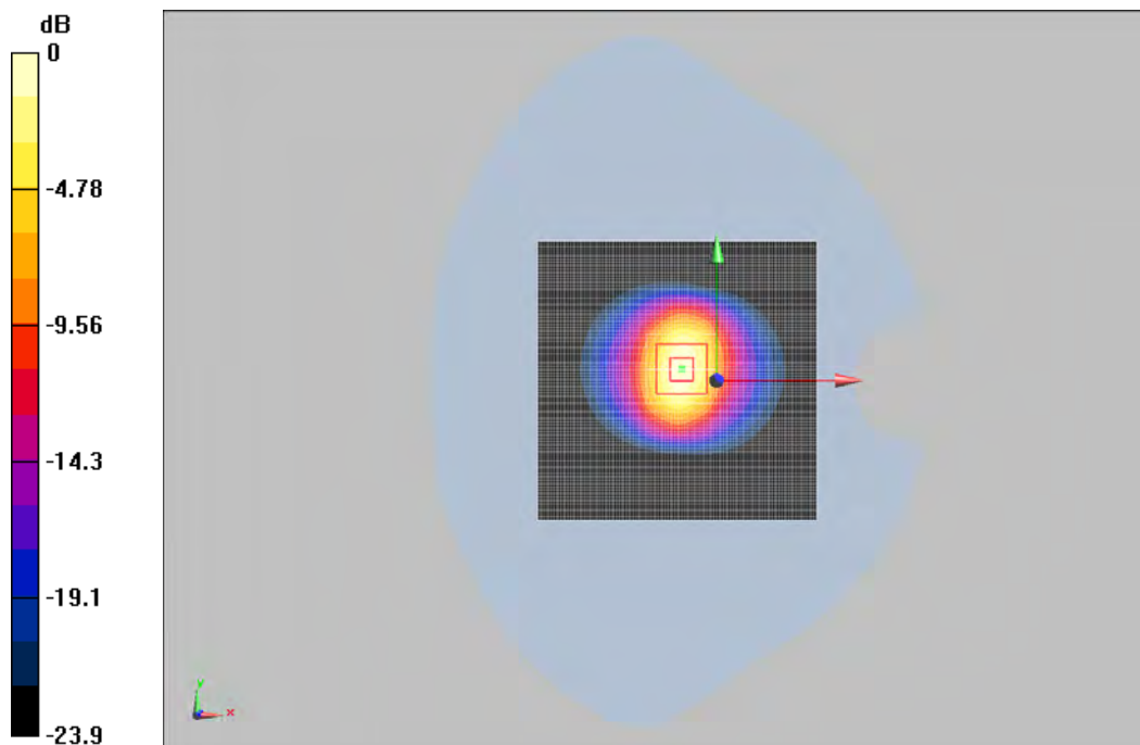
0 dB = 15.8W/kg
