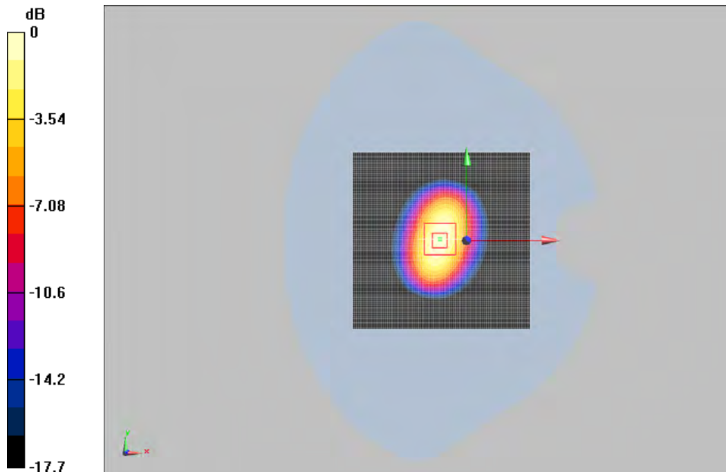
0 dB = 11.7W/kg
