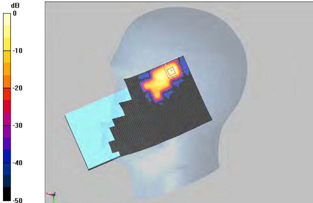
0 dB = 0.175W/kg
