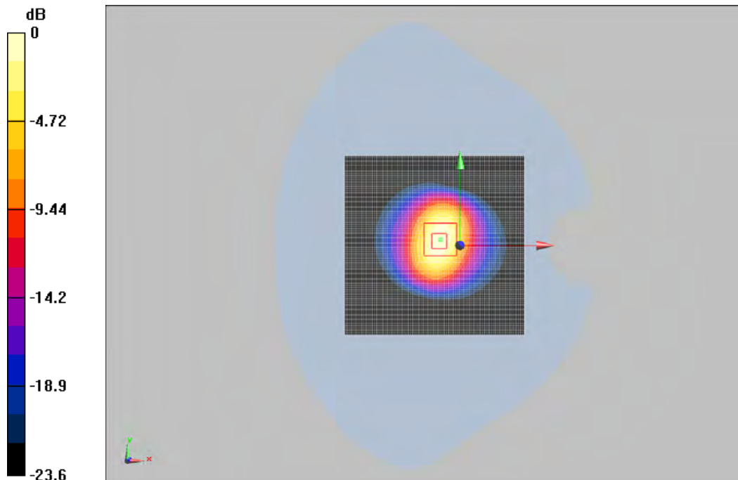
0 dB = 15.6W/kg
