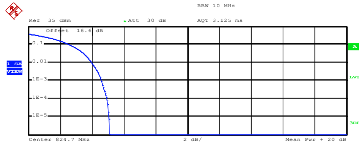
Peak-to-Average Ratio on Channel 1013 (824.70 MHz)
