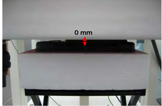
Fig.9 EUT with mobile battery back side to flat phantom
