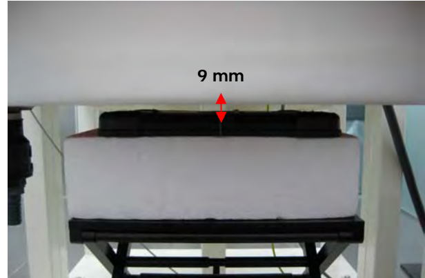
Fig.7 EUT Back side mode to flat phantom
