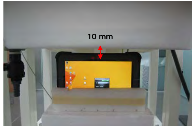
Fig.8 EUT Top side to flat phantom
