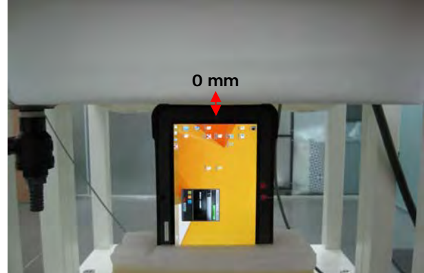
Fig.5 EUT Left side to flat phantom
