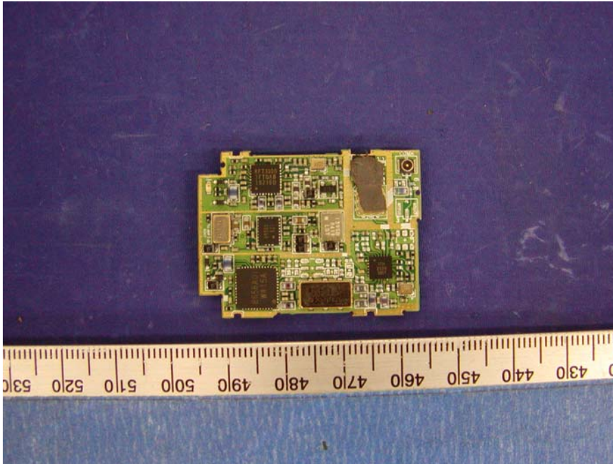
EUT – Transmitter Board Cover Removed View
