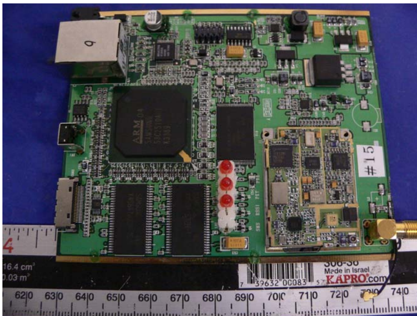
EUT – Component without Shielding View
