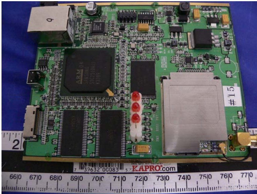
EUT – Component with Shielding View
