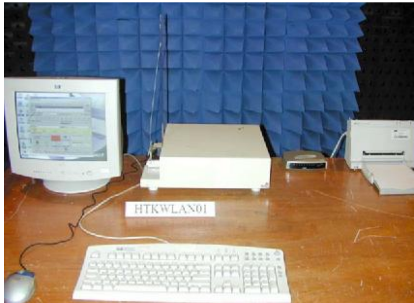
Photo 1: Spurious Test Set-up (front)
