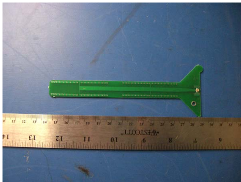
Antenna photo
