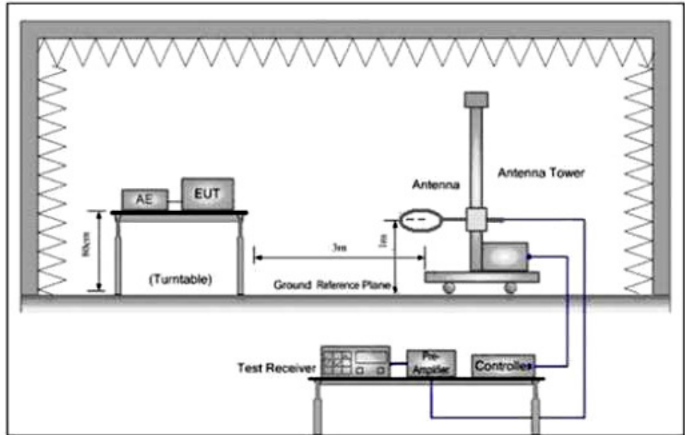
Figure 1. Below 30MHz
