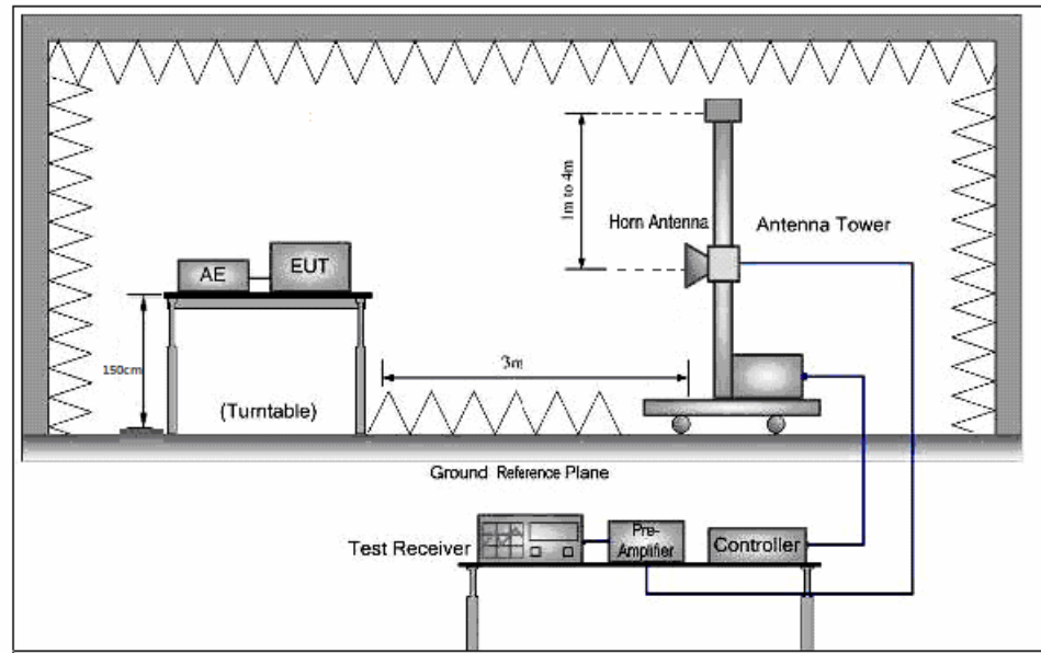
Figure 3. Above 1 GHz
