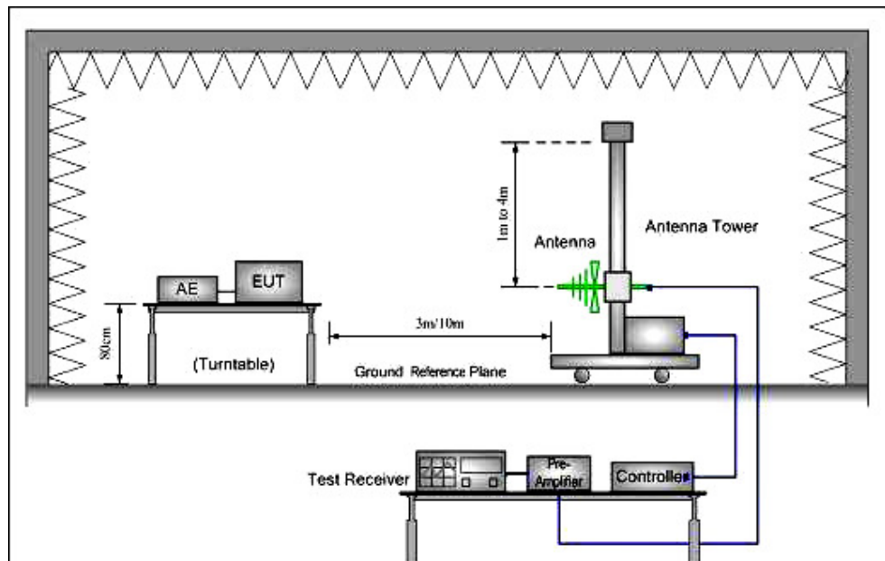
Figure 2. 30MHz to 1GHz
